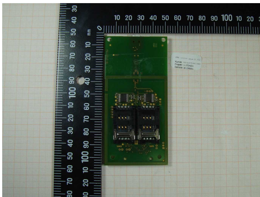
Photo 4: EUT with dummy antenna for AC conducted emission tests
