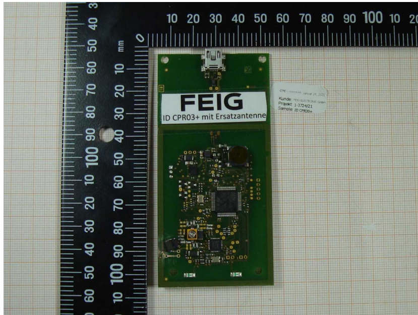
Photo 3: EUT with dummy antenna for AC conducted emission tests
