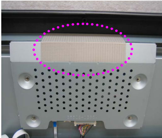
3. Attached the shield tape
