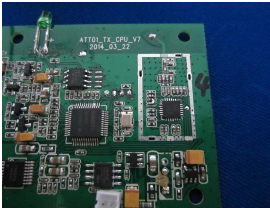
EUT- Main Board Top Shielding Off View
