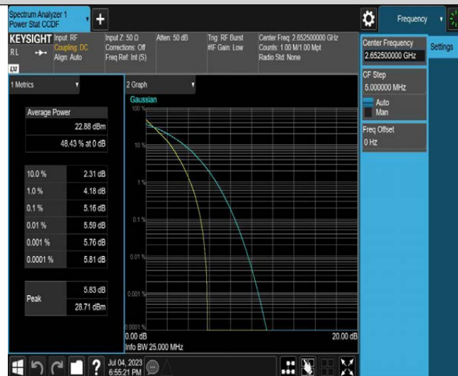
Band41-5MHz-QPSK-41215-25RB#0
