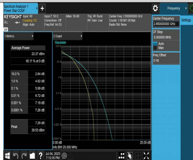
Band41-15MHz-QPSK-40115-75RB#0
