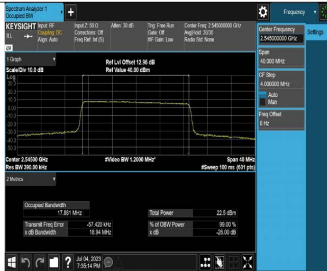
Band41-20MHz-16QAM-40640-100RB#0
