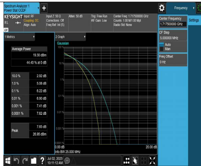
Band10-15MHz-16QAM-22450-75RB#0
