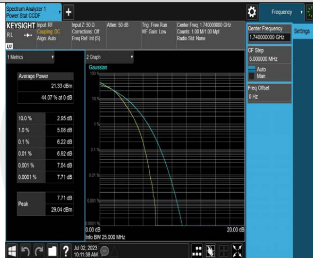
Band10-15MHz-16QAM-22675-75RB#0
