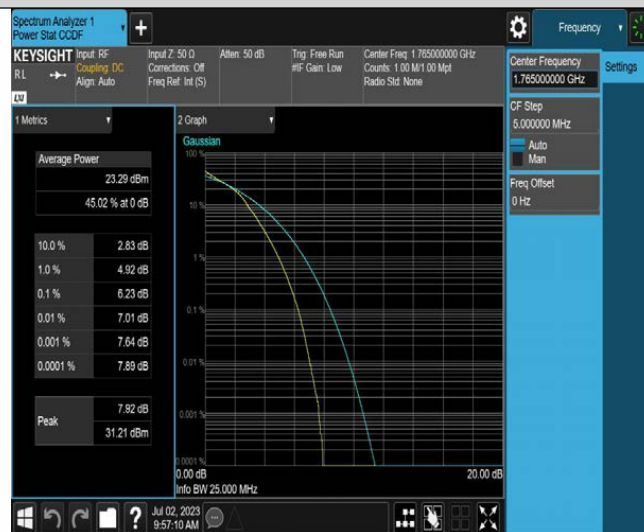
Band10-15MHz-QPSK-22225-75RB#0
