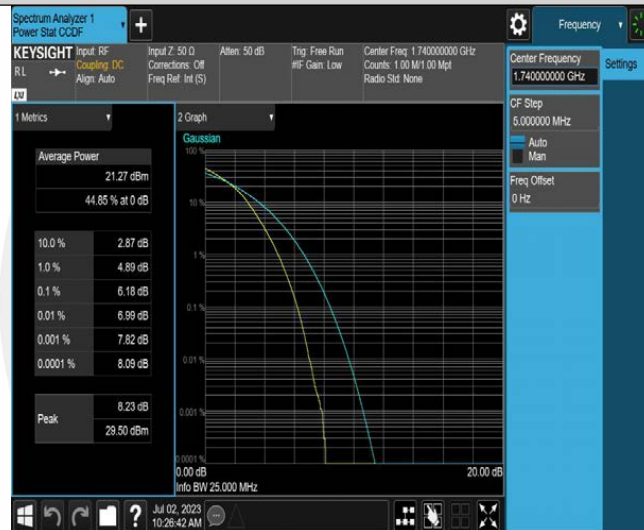
Band10-20MHz-16QAM-22650-100RB#0
