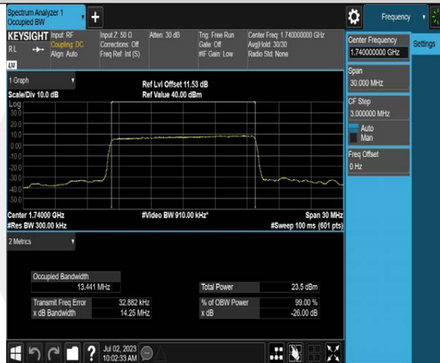
Band 10-15MHz-QPSK-22675-75RB#0
