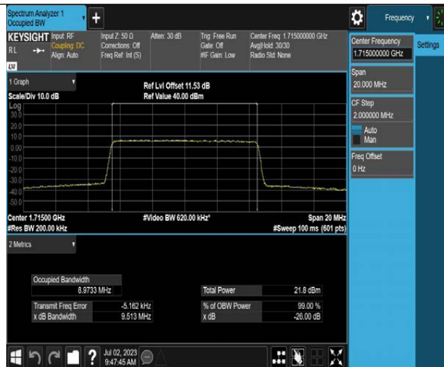
Band10-10MHz-QPSK-22450-50RB#0
