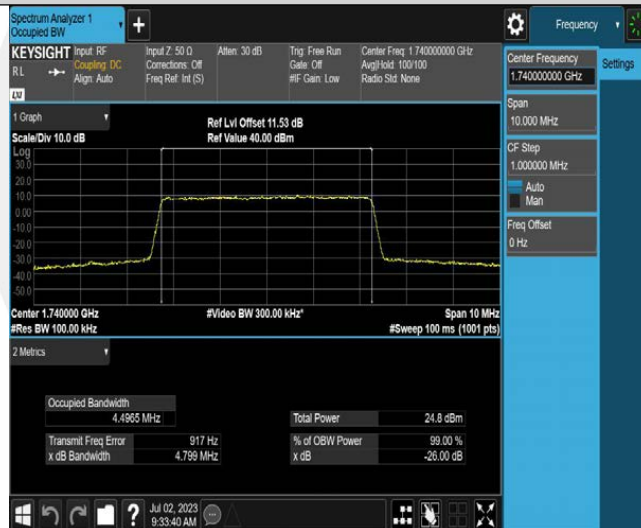
Band10-5MHz-QPSK-22725-25RB#0
