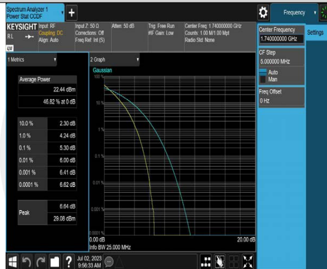
Band10-10MHz-QPSK-22700-50RB#0
