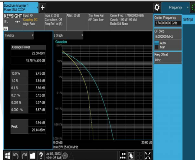
Band10-15MHz-QPSK-22675-75RB#0
