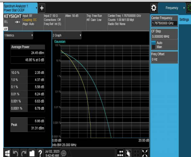
Band10-5MHz-QPSK-22725-25RB#0
