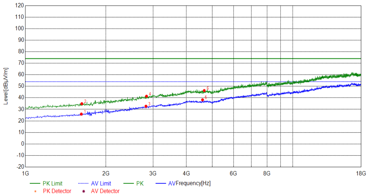
(Plot M: Test Antenna Horizontal 1G – 18G)
