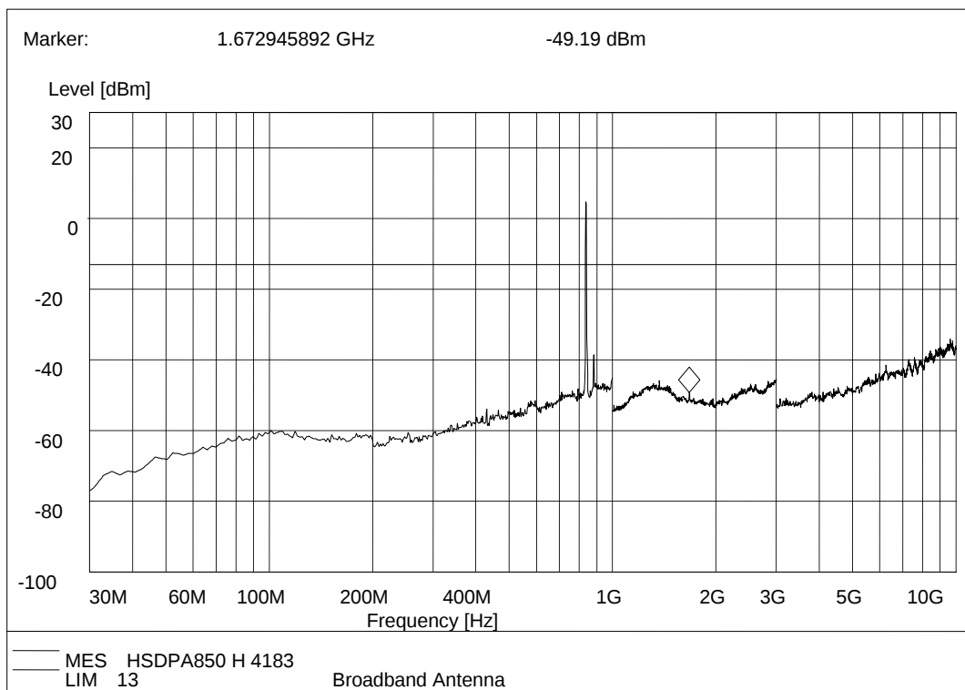
(Plot I.3: HSDPA 850MHz Channel = 4183, Test Antenna Horizontal)
