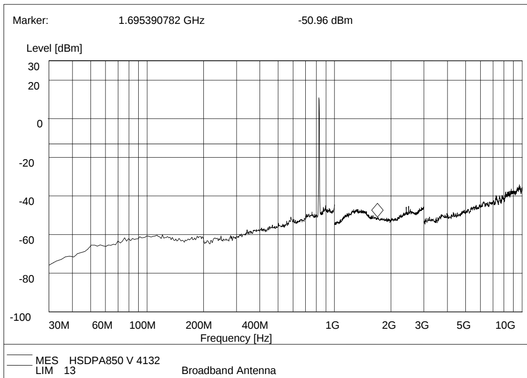
(Plot I.2: HSDPA 850MHz Channel = 4132, Test Antenna Vertical)
