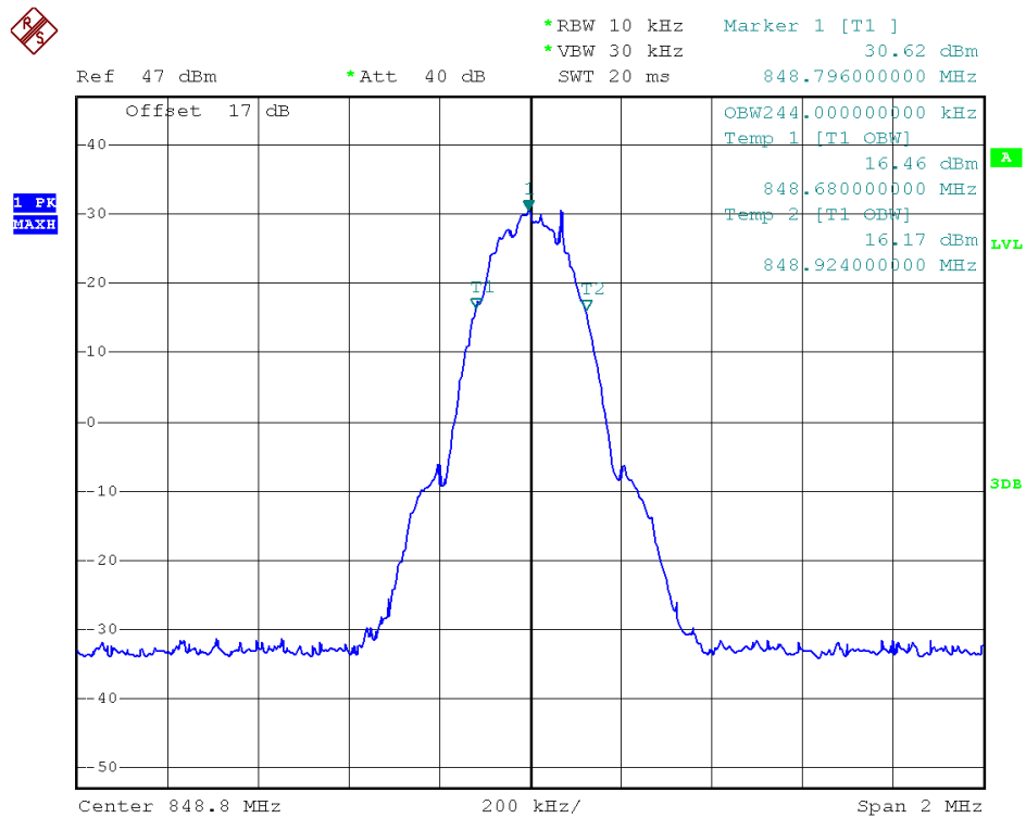
(Plot A1: EDGE 850MHz Channel = 251)
