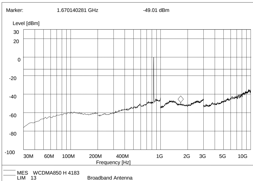
(Plot G.3: WCDMA 850MHz Channel = 4183, Test Antenna Horizontal)
