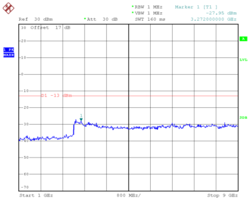
(Plot G1.1: HSDPA 850MHz Channel = 4132, 1GHz to 9GHz)
