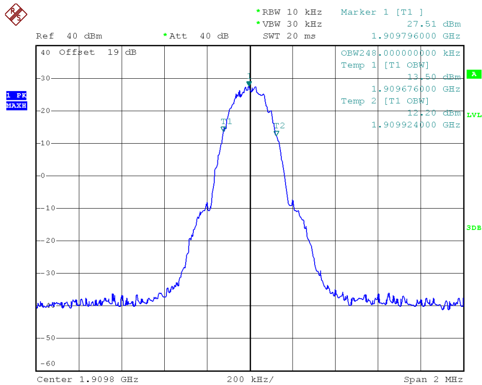
(Plot X: GPRS 1900MHz Channel = 810)
