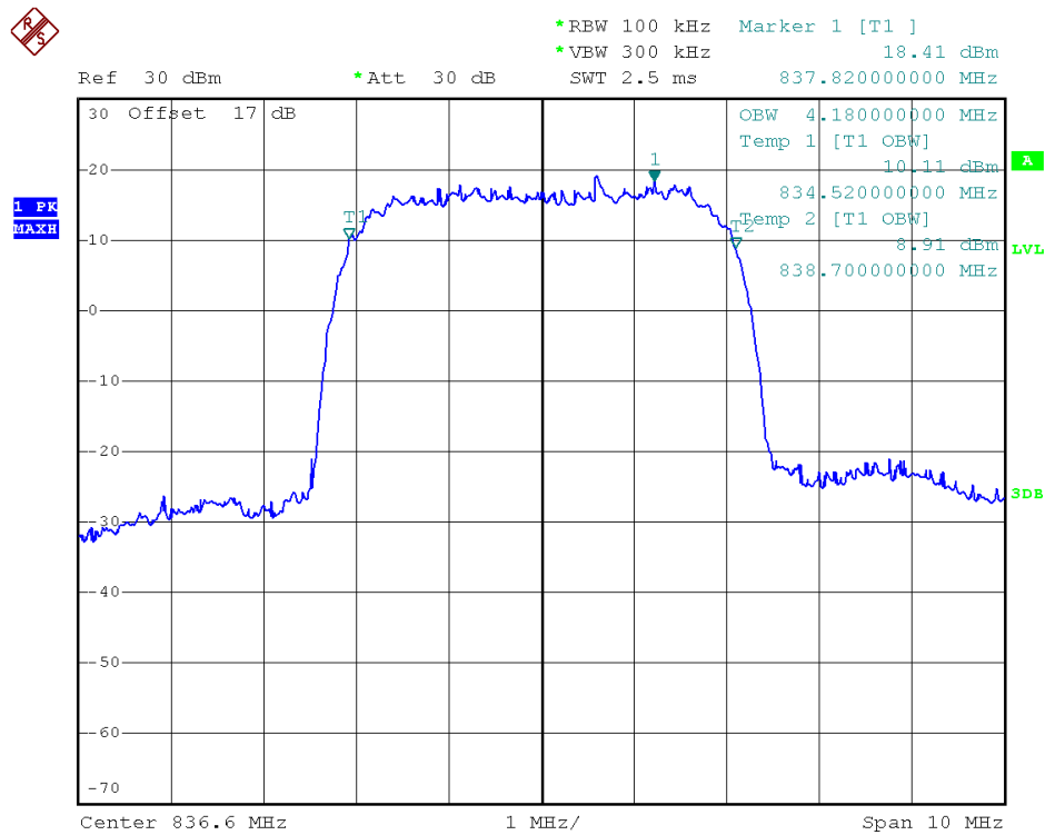
(Plot H: HSDPA850 MHz Channel = 4183)
