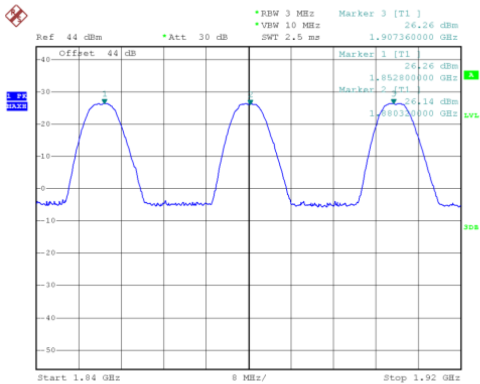
(Plot J: HSDPA1900 MHz Channel = 9262, 9400, 9538)
