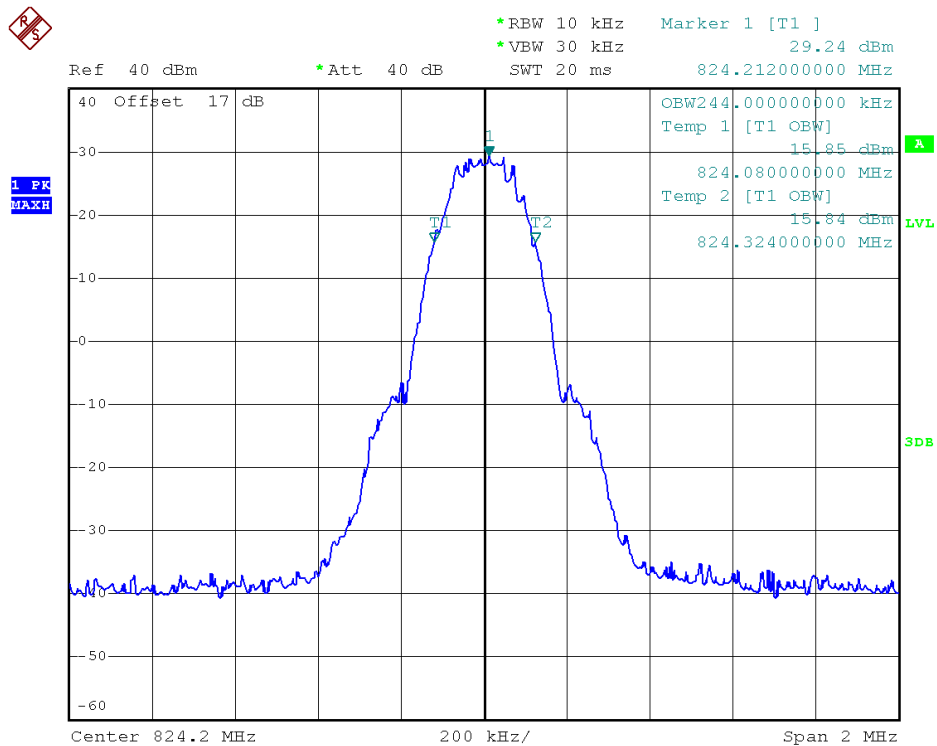
(Plot S: GPRS 850MHz Channel = 128)
