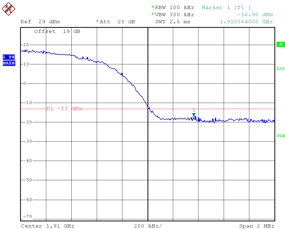
(Plot P: HSDPA 1900 Channel = 9538)
