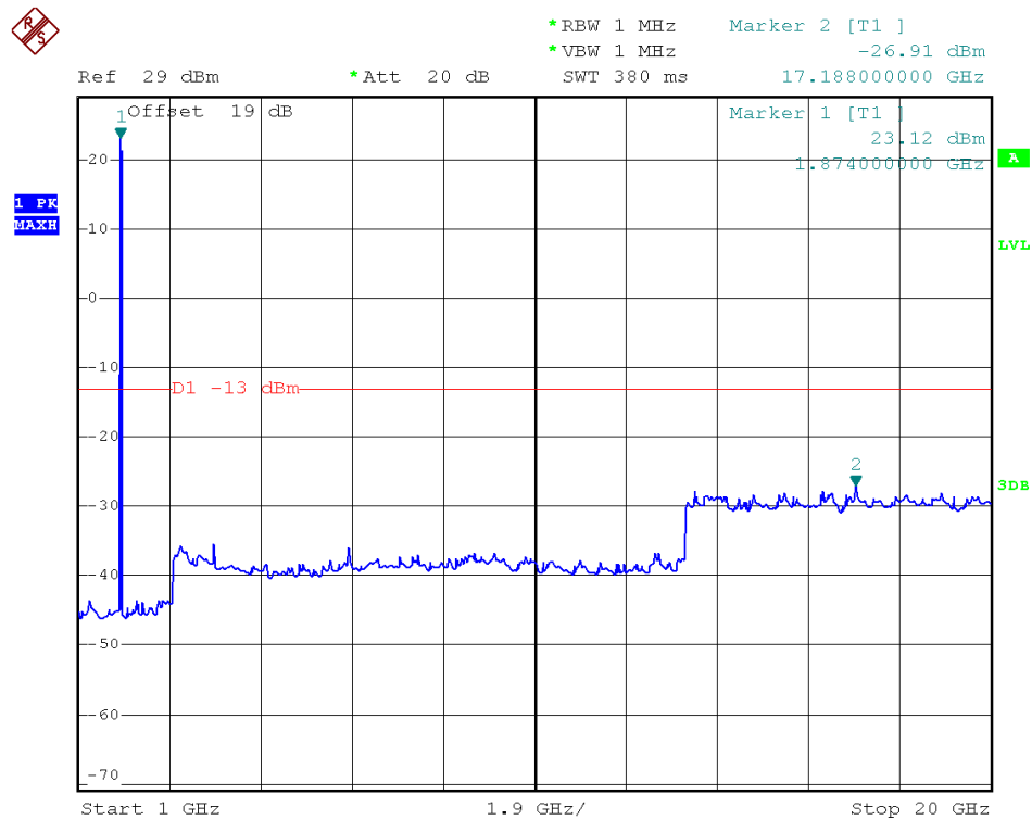
(Plot H3.1: HSDPA1900MHz Channel = 9538 1GHz to 20GHz)
