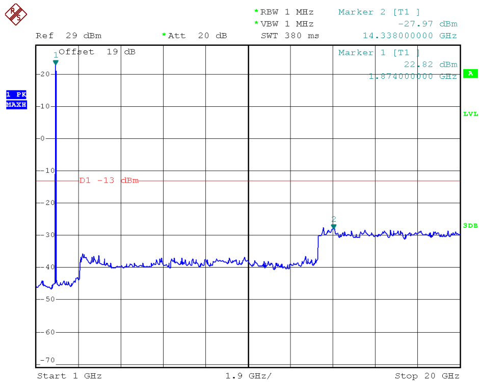
(Plot H2.1: HSDPA1900MHz Channel = 9400, 1GHz to 20GHz)
