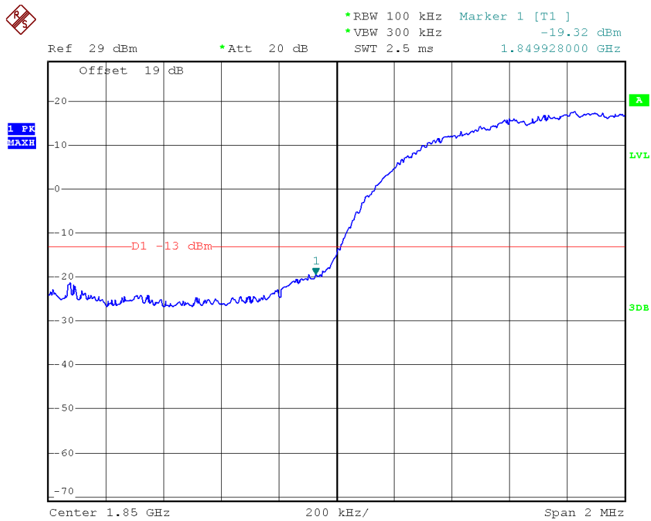
(Plot O: HSDPA 1900 Channel = 9262)
