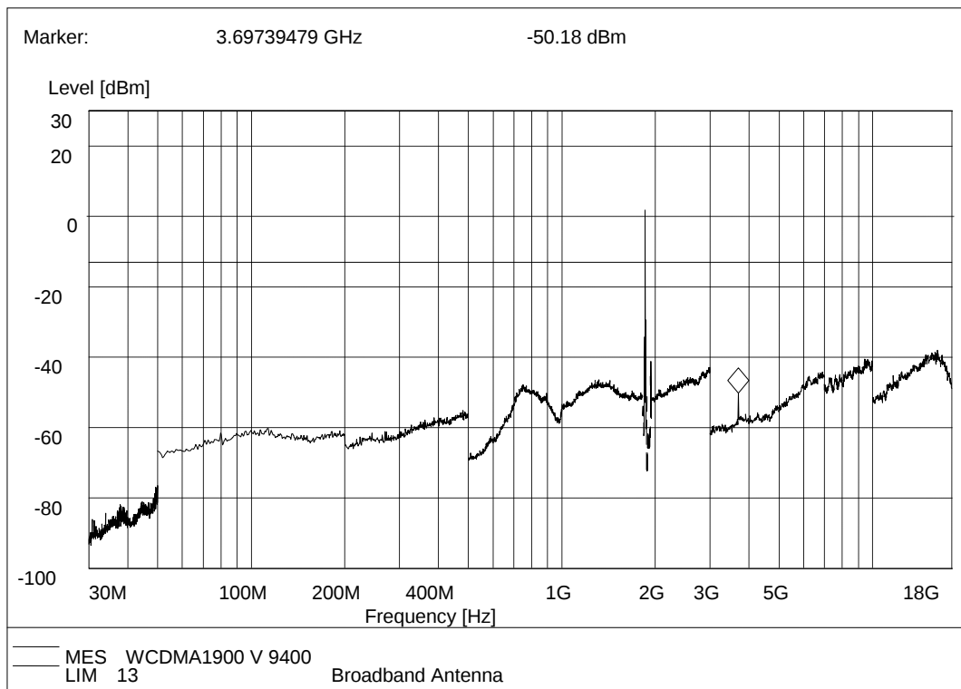
(Plot H.4: WCDMA 1900MHz Channel = 9400, Test Antenna Vertical)
