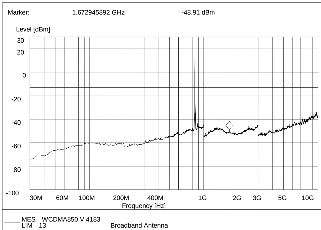
(Plot G.4: WCDMA 850MHz Channel = 4183, Test Antenna Vertical)
