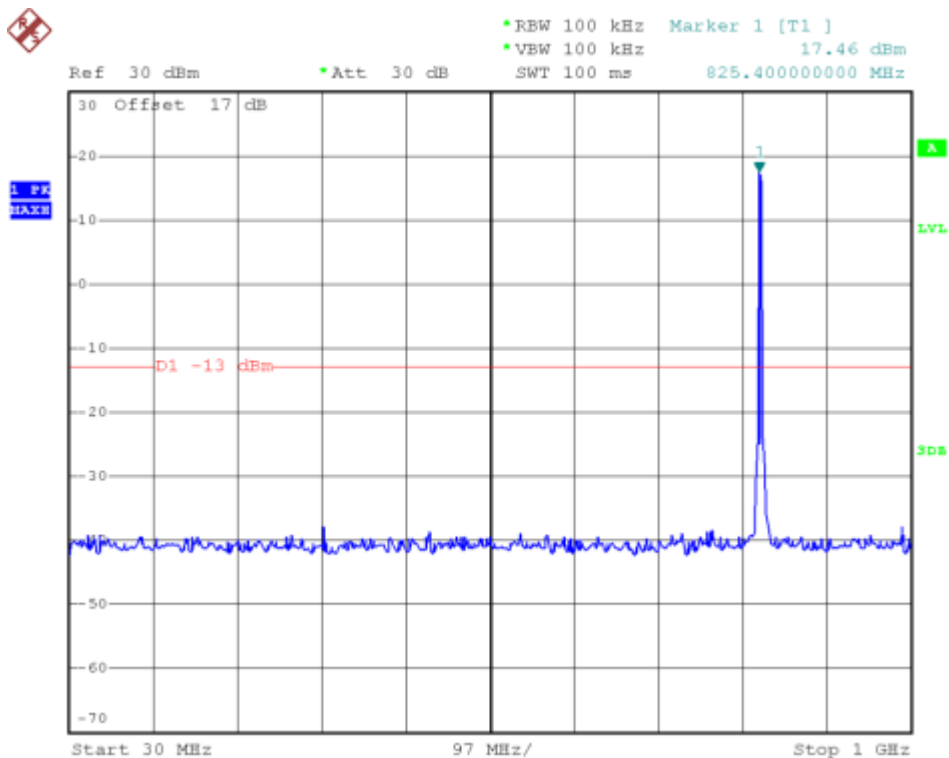
(Plot G1: HSDPA 850MHz Channel = 4132, 30MHz to 1GHz)
