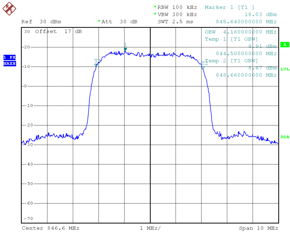
(Plot C: WCDMA 850MHz Channel = 4233)
