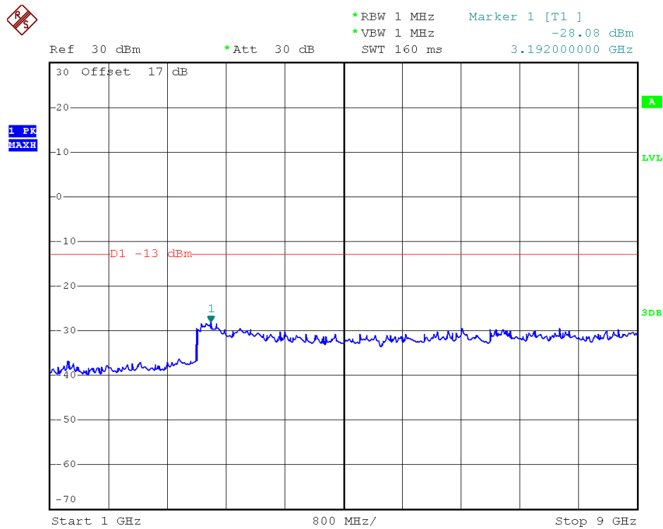
(Plot G2.1: HSDPA 850MHz Channel = 4183, 1GHz to 9GHz)
