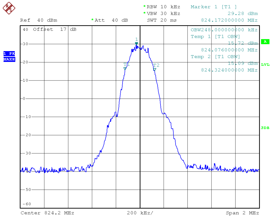
(Plot M: GSM 850MHz Channel = 128)
