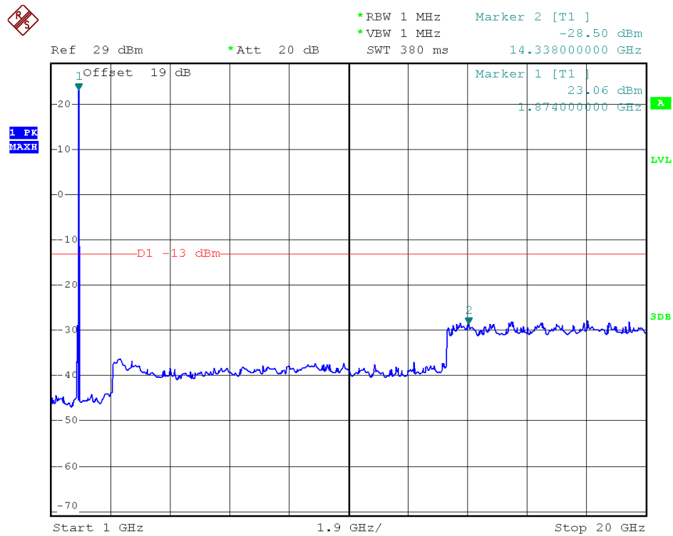
(Plot H1.1: HSDPA1900MHz Channel = 9262, 1GHz to 20GHz)
