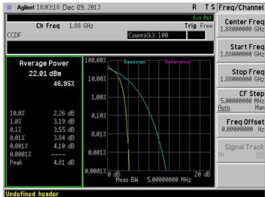
(Plot D2: HSDPA 1900MHz Channel = 9400)
