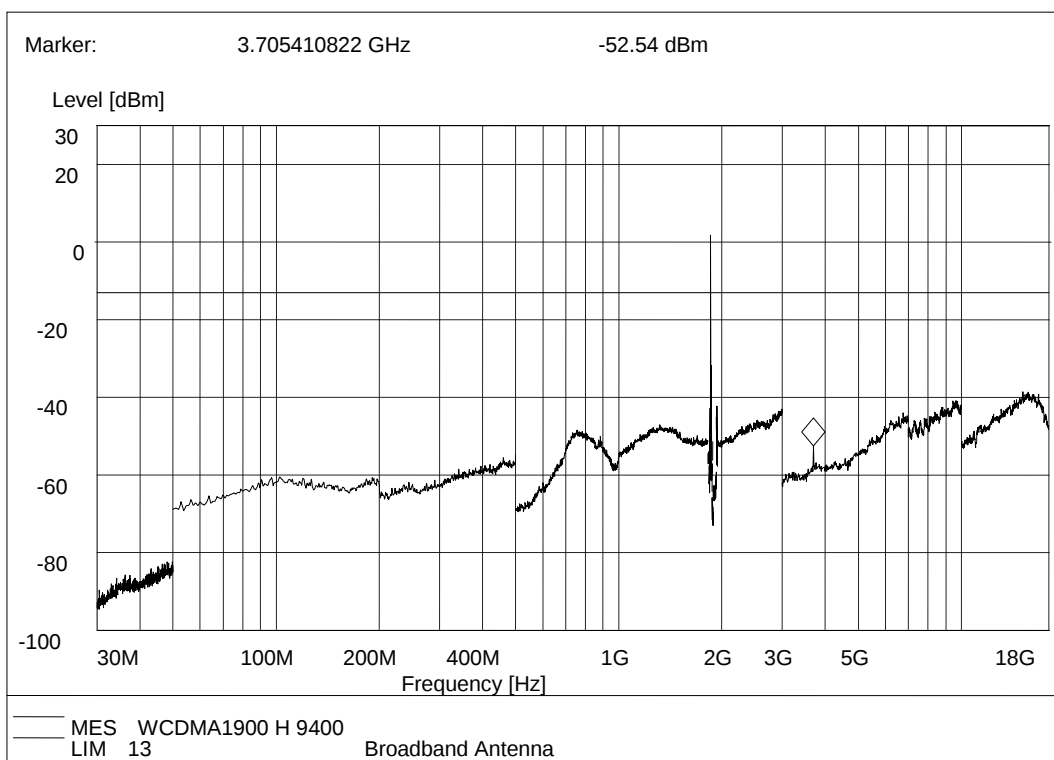
(Plot H.3: WCDMA 1900MHz Channel = 9400, Test Antenna Horizontal)
