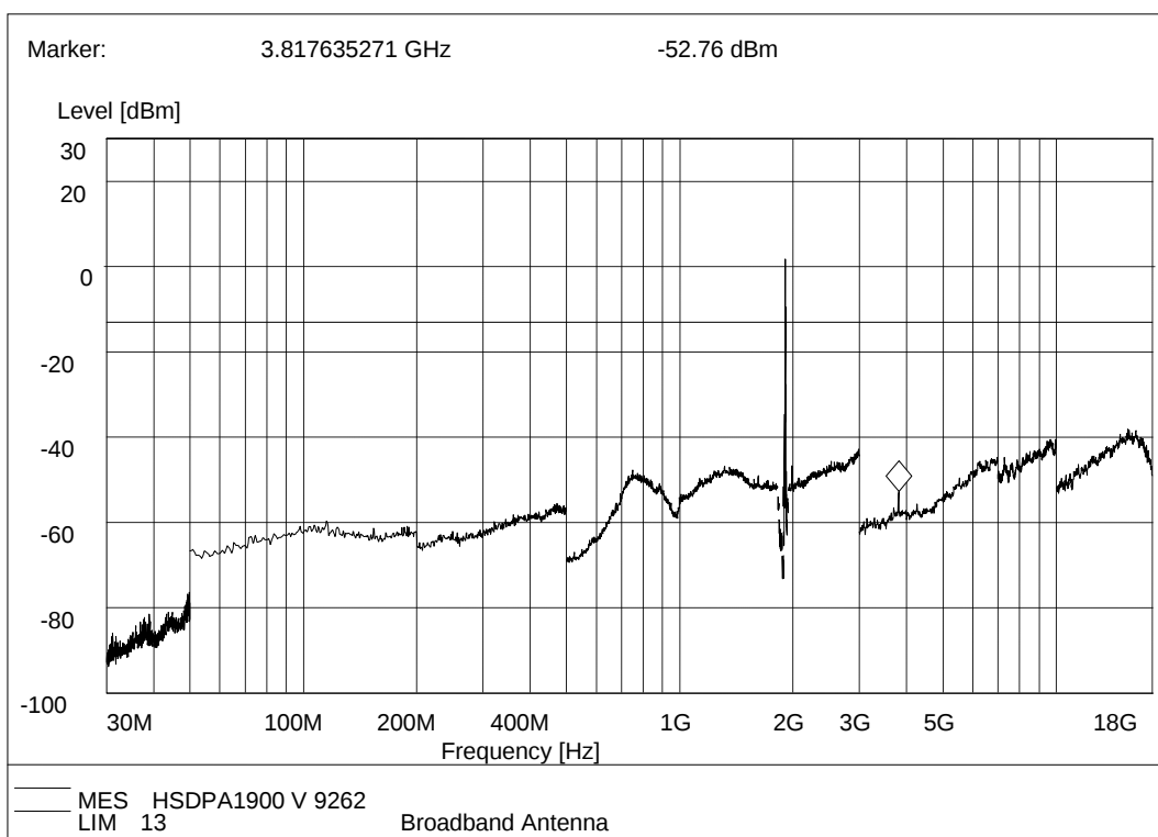
(Plot J.2: HSDPA 1900 MHz Channel = 9262, Test Antenna Vertical)
