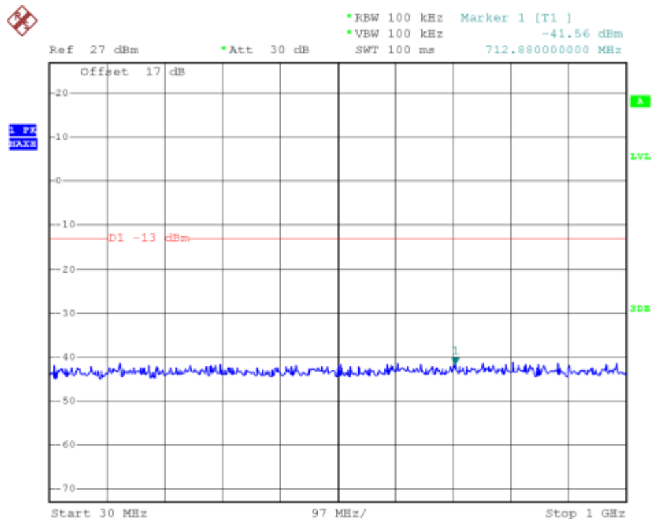
(Plot H3: HSDPA1900MHz Channel = 9538, 30MHz to 1GHz)
