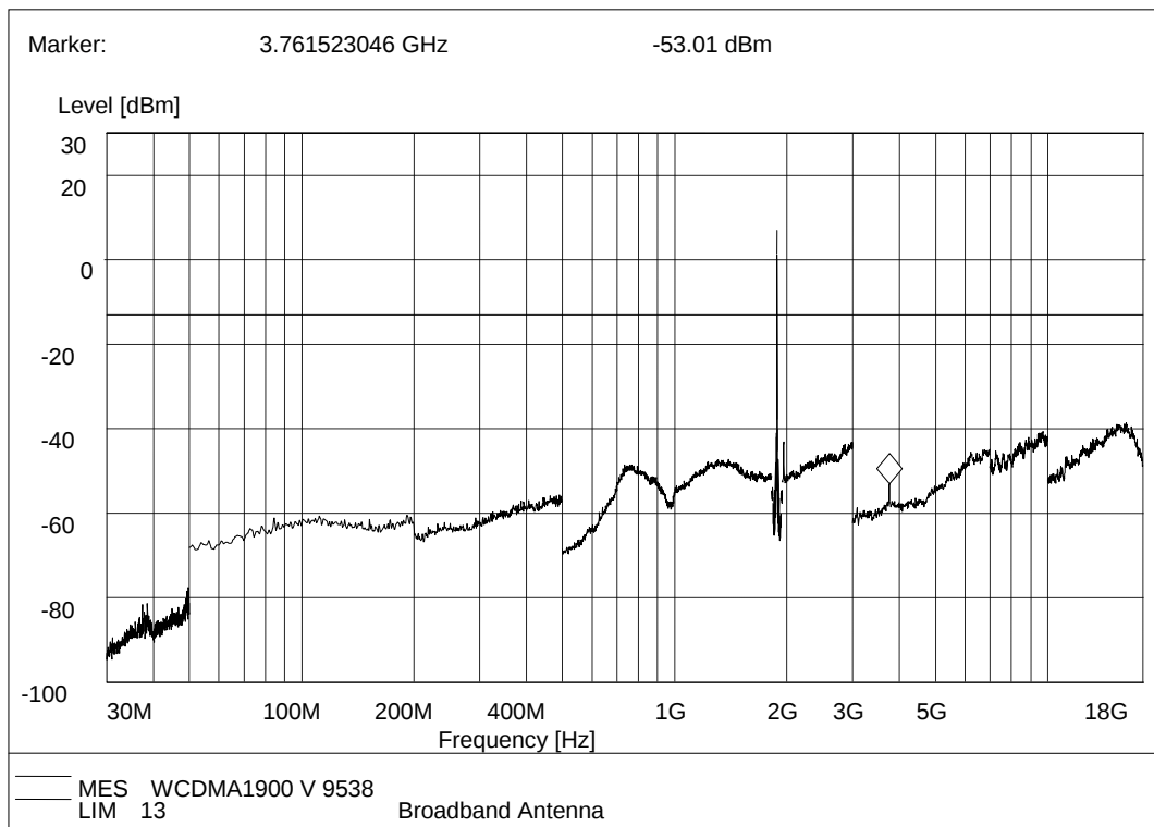
(Plot H.6: WCDMA 1900MHz Channel = 9538, Test Antenna Vertical)
