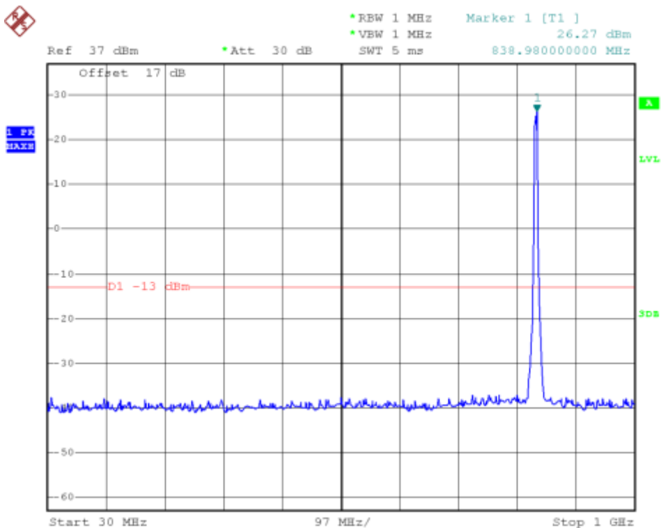
(Plot G2: HSDPA 850MHz Channel = 4183, 30MHz to 1GHz)
