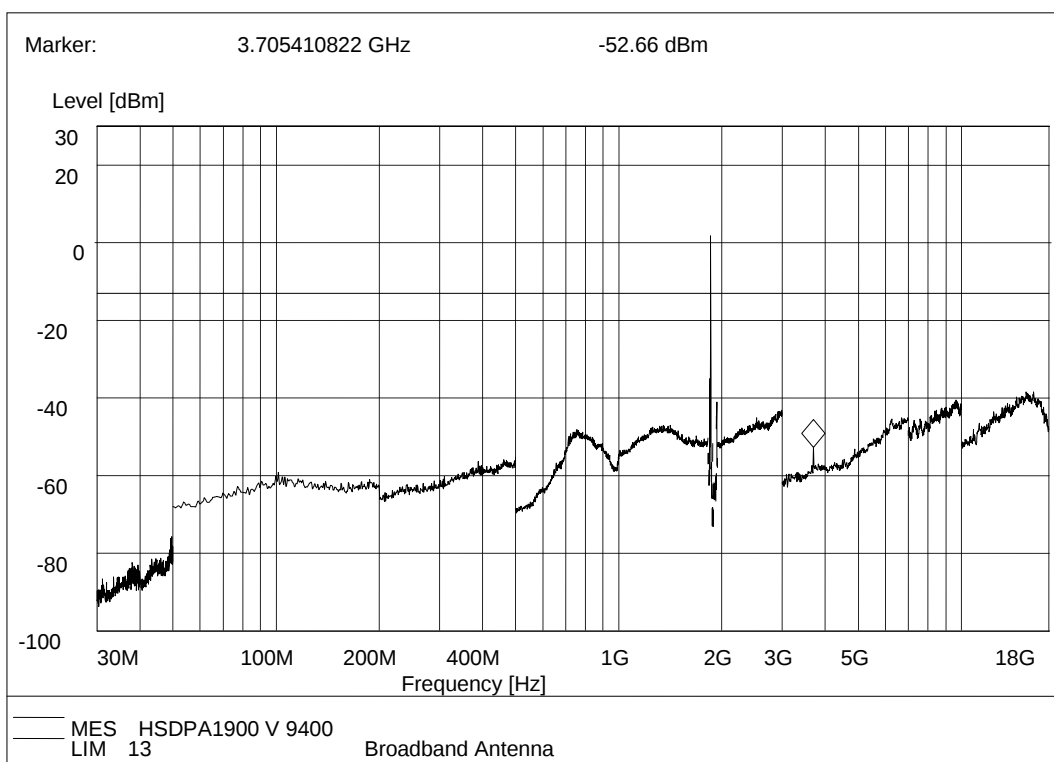
(Plot J.4: HSDPA 1900 MHz Channel = 9400, Test Antenna Vertical)
