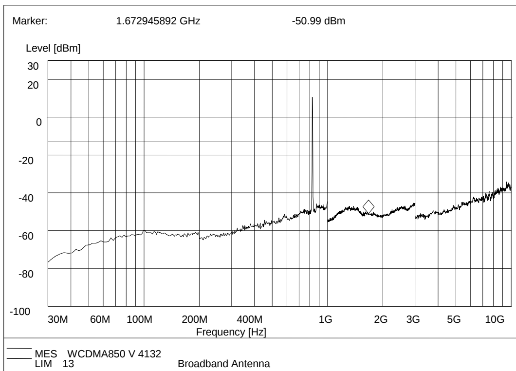
(Plot G.2: WCDMA 850MHz Channel = 4132, Test Antenna Vertical)
