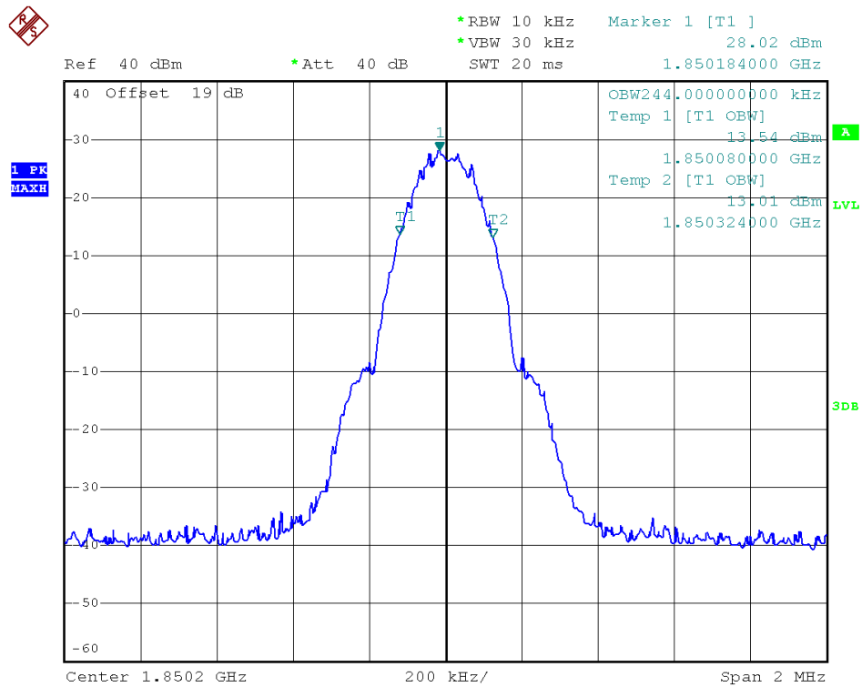
(Plot P: GSM 1900MHz Channel = 512)
