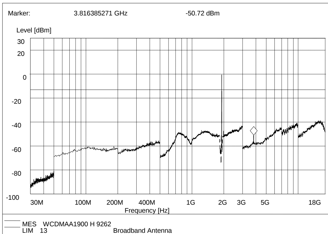
(Plot H.1: WCDMA 1900MHz Channel = 9262, Test Antenna Horizontal)
