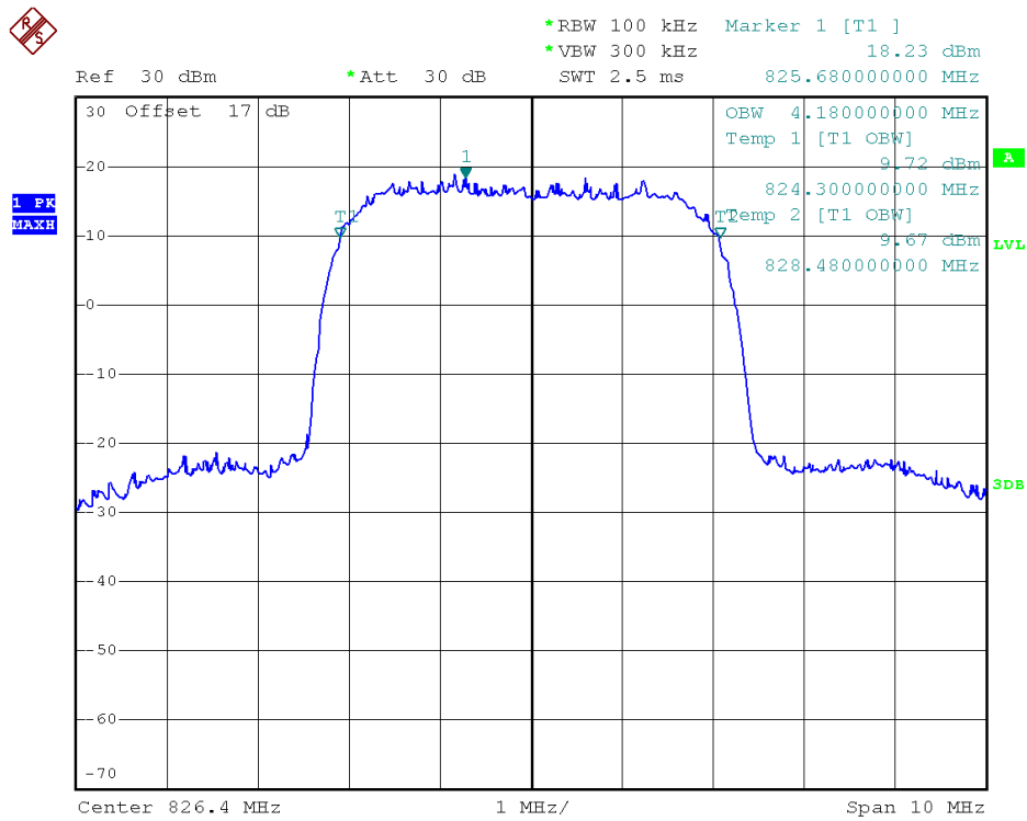
(Plot G: HSDPA 850MHz Channel = 4132)
