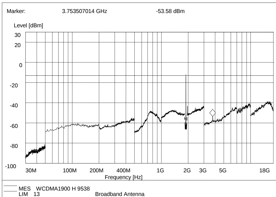
(Plot H.5: WCDMA 1900MHz Channel = 9538, Test Antenna Horizontal)
