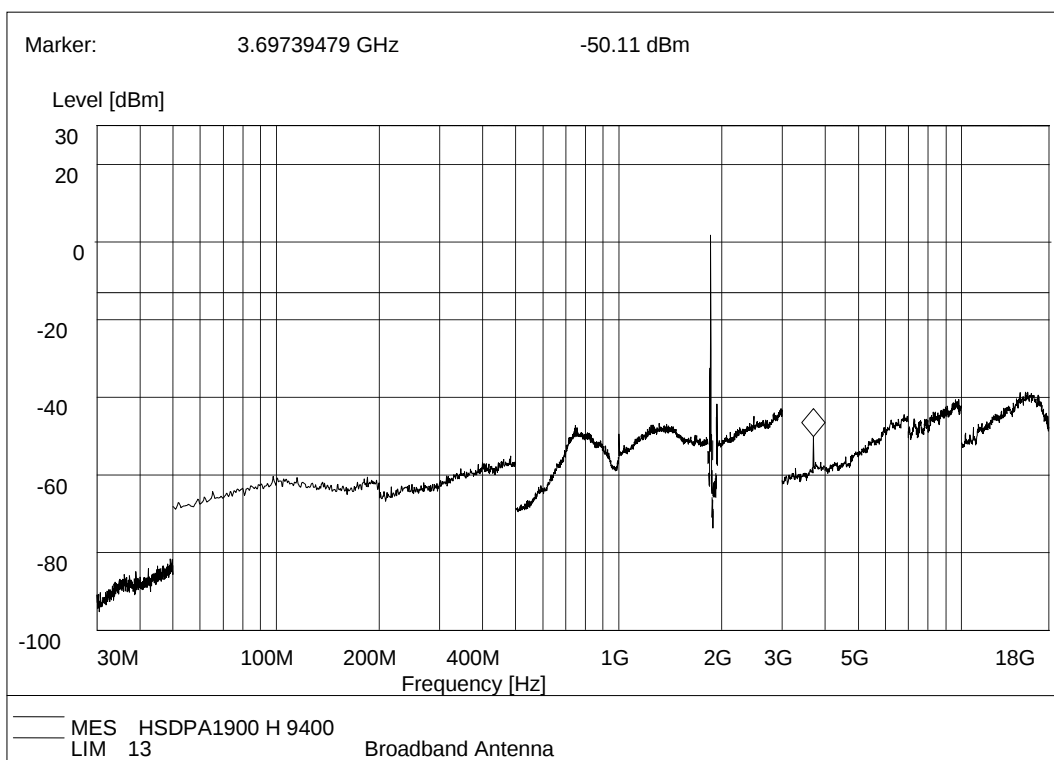
(Plot J.3: HSDPA 1900 MHz Channel = 9400, Test Antenna Horizontal)
