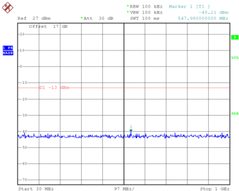
(Plot H2: HSDPA1900MHz Channel = 9400, 30MHz to 1GHz)
