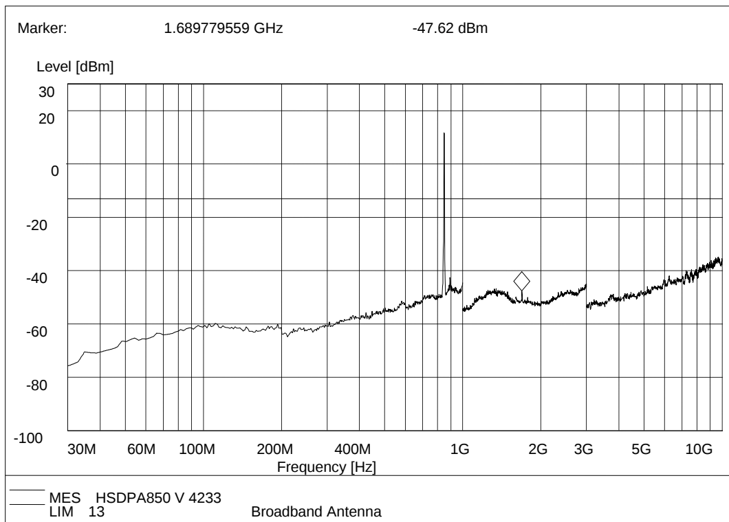
(Plot I.6: HSDPA 850MHz Channel = 4233, Test Antenna Vertical)
