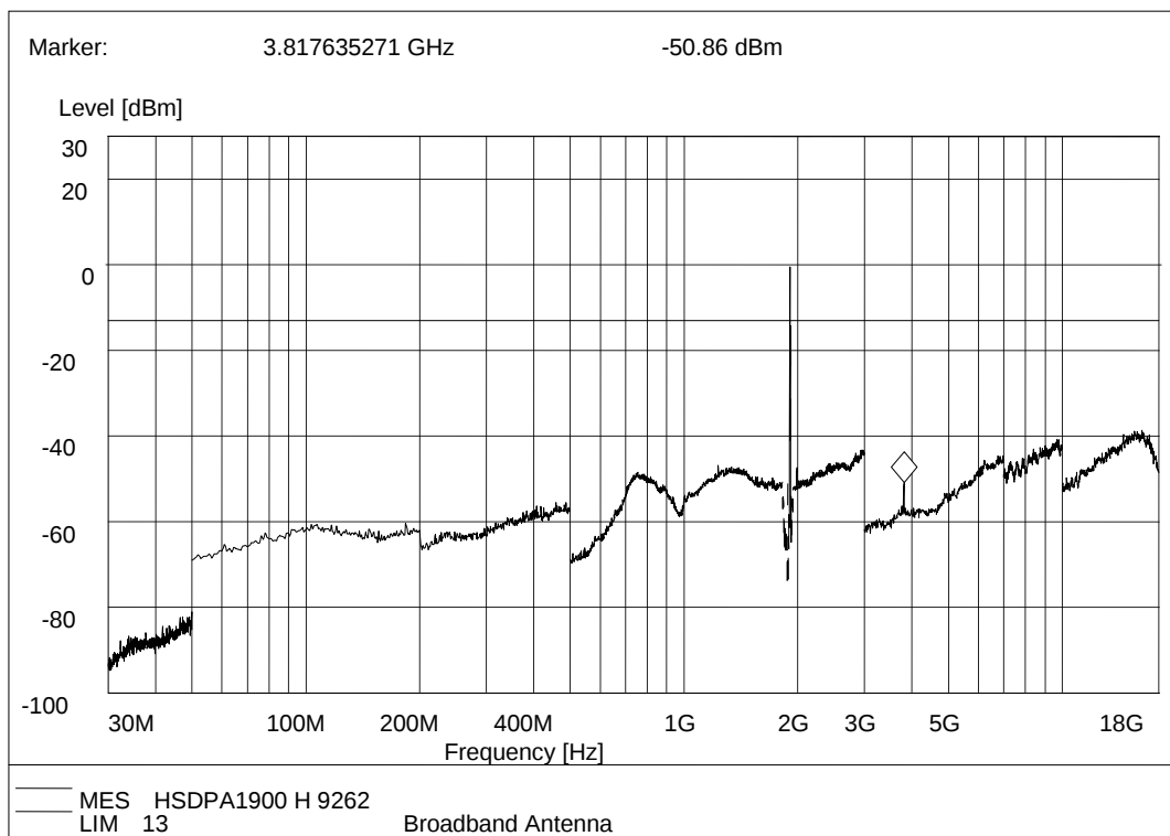
(Plot J.1: HSDPA 1900 MHz Channel = 9262, Test Antenna Horizontal)
