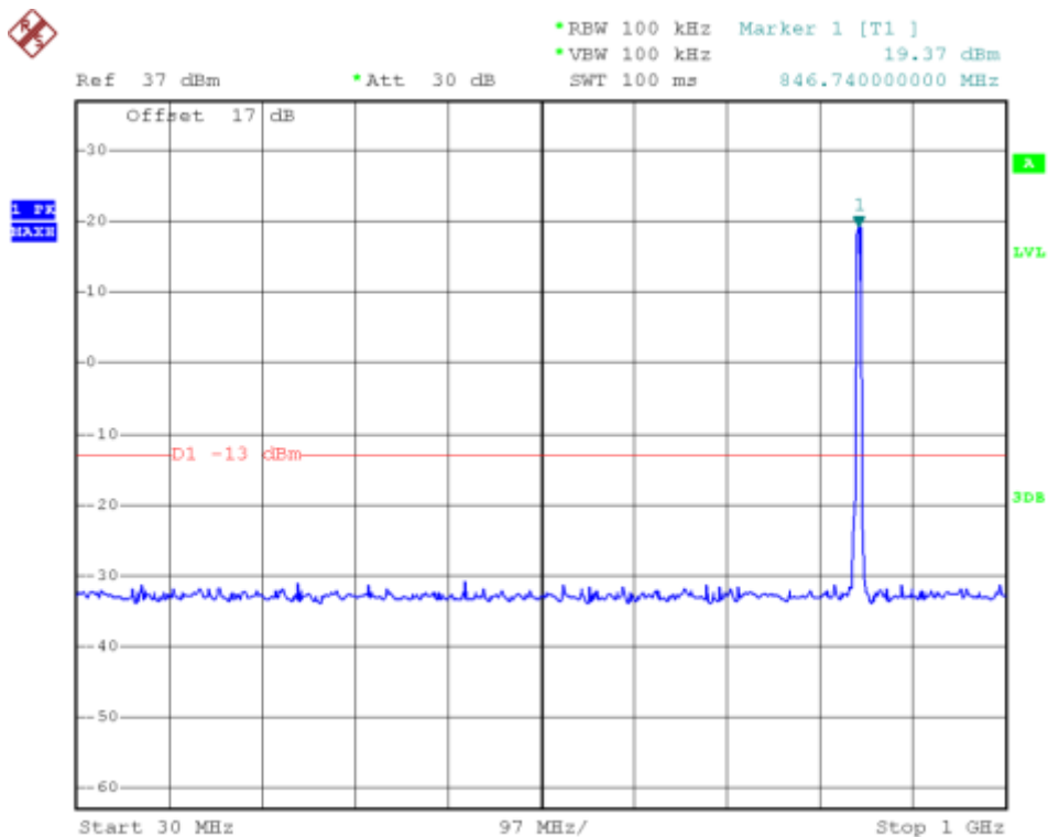
(Plot G3: HSDPA850MHz Channel = 4233, 30MHz to 1GHz)
