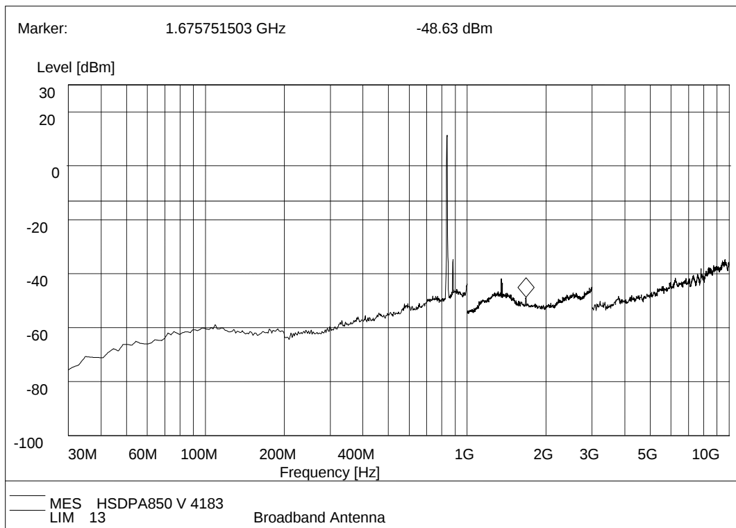
(Plot I.4: HSDPA 850MHz Channel = 4183, Test Antenna Vertical)
