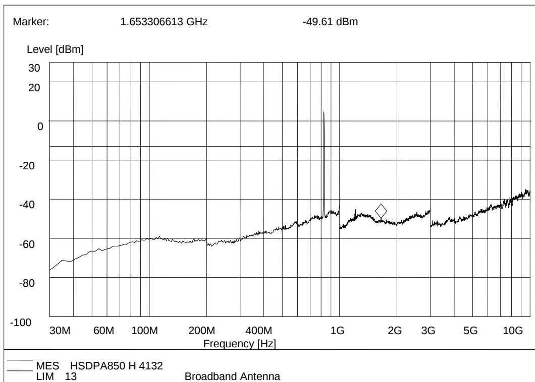
(Plot I.1: HSDPA 850MHz Channel = 4132, Test Antenna Horizontal)
