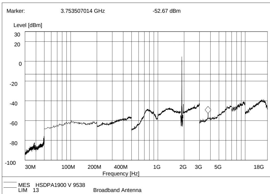
(Plot J.6: HSDPA 1900 MHz Channel = 9538, Test Antenna Vertica
