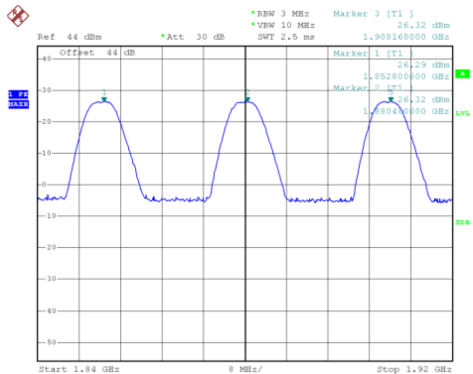
(Plot I: WCDMA 1900 MHz Channel = 9262, 9400, 9538)
