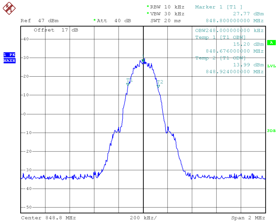
(Plot U: GPRS850MHz Channel = 251)
