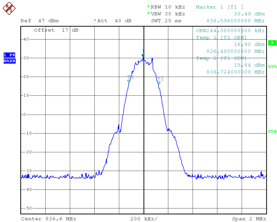
(Plot T: GPRS 850MHz Channel = 190)
