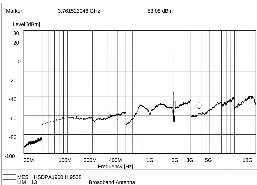
(Plot J.5: HSDPA 1900 MHz Channel = 9538, Test Antenna Horizontal)
