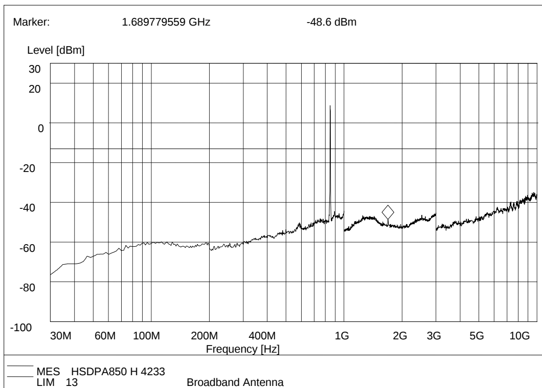
(Plot I.5: HSDPA 850MHz Channel = 4233, Test Antenna Horizontal)
