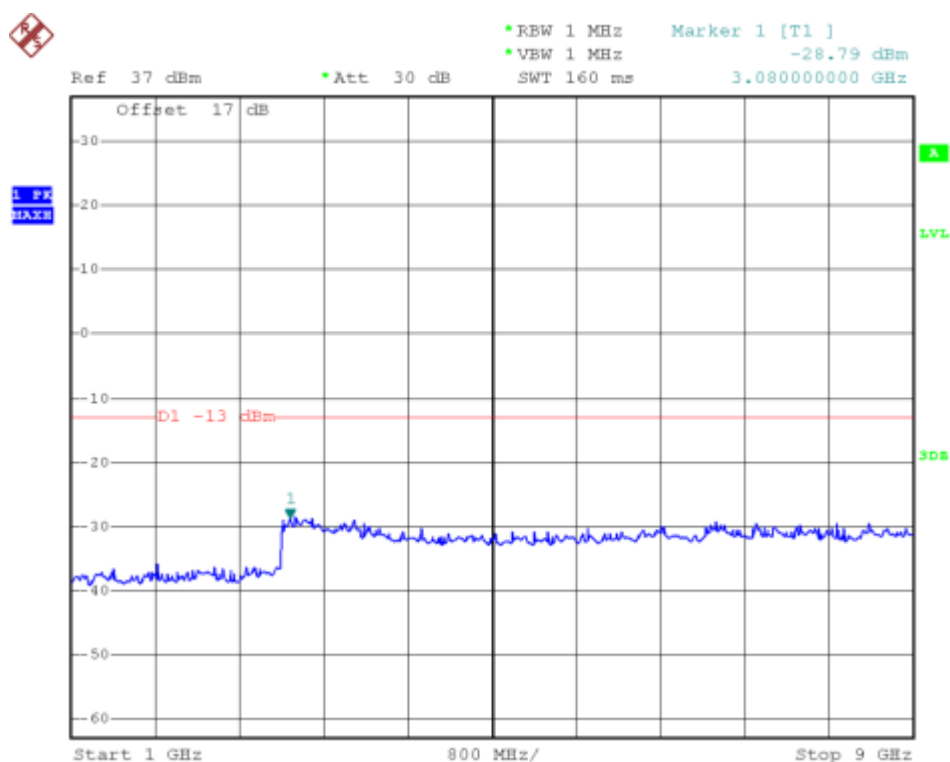
(Plot G3.1: HSDPA850MHz Channel = 4233, 1GHz to 9GHz)
