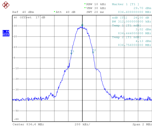
(Plot H: GPRS 850MHz Channel = 190)
