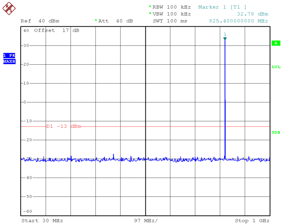
(Plot A1: GSM 850MHz Channel = 128, 30MHz to 1GHz)
