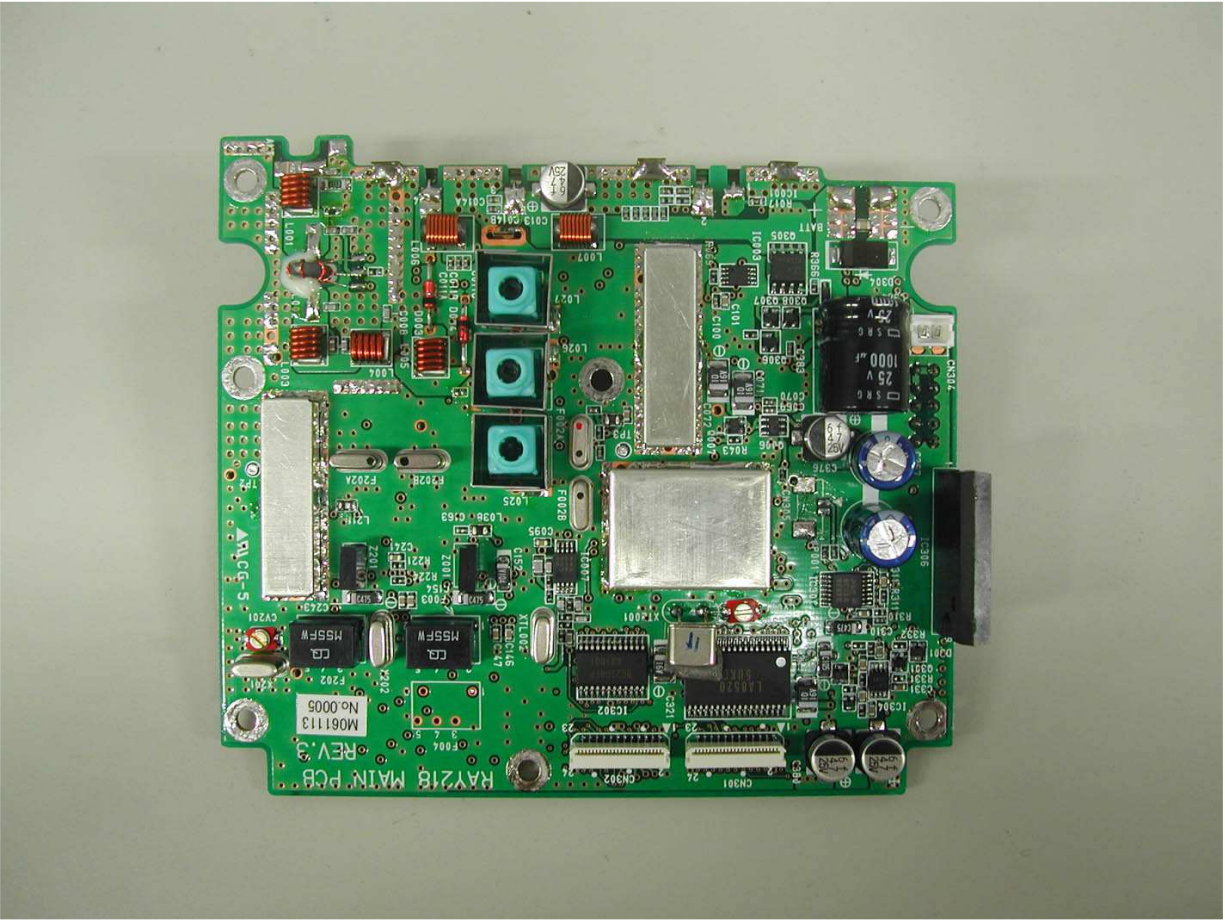
Main PCB -1
