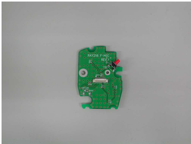
Hand Mic PCB 1
