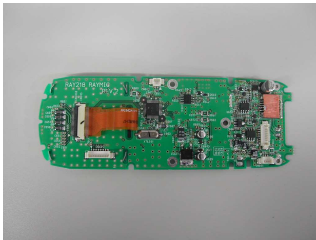
RayMic PCB-2
