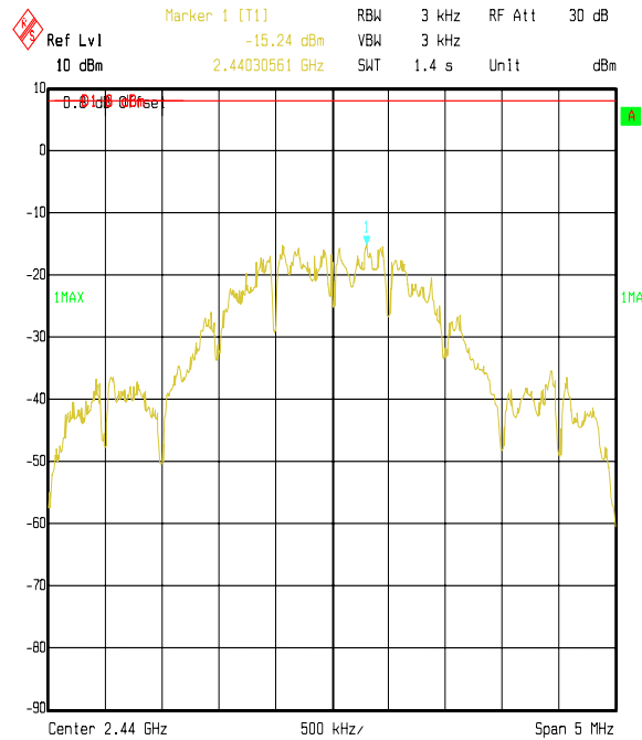
Title: Raymarine EUT: Smart Controller. Spectral Dens FCC P15.247 Comment A: 46813 Middle Channel Date: 24.NOV.2004 13:53:41
