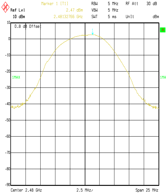
Title: Raymarine EUT: Smart Controller. Peak Power FCC P15.247 Comment A: 46813 Top Channel Date: 24.NOV.2004 13:28:32
