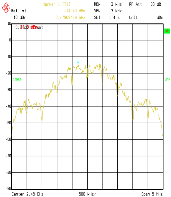
Title: Raymarine EUT: Smart Controller. Spectral Dens FCC P15.247 Comment A: 46813 Top Channel Date: 24.NOV.2004 13:50:53
