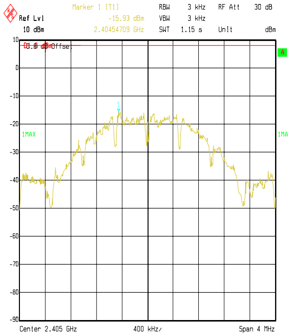
Title: Raymarine EUT: Smart Controller. Spectral Dens FCC P15.247 Comment A: 46813 Bottom Channel Date: 24.NOV.2004 14:04:30
