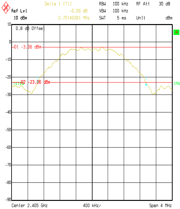
Title: Raymarine EUT: Smart Controller. 20dB Bandwidth FCC P15.247 Comment A: 46813 Bottom Channel Date: 24.NOV.2004 14:03:19
