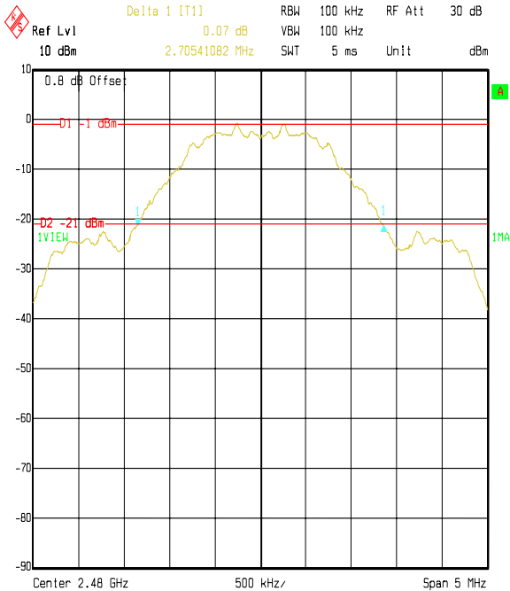
Title: Raymarine EUT: Smart Controller. 20dB Bandwidth FCC P15.247 Comment A: 46813 Top Channel Date: 24.NOV.2004 13:49:42
