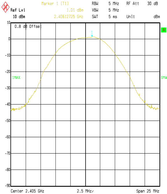
Title: Raymarine EUT: Smart Controller. Peak Power FCC P15.247 Comment A: 46813 Bottom Channel Date: 24.NOV.2004 14:05:03
