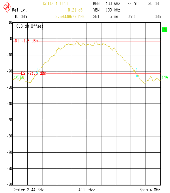
Title: Raymarine EUT: Smart Controller. 20dB Bandwidth FCC P15.247 Comment A: 46813 Middle Channel Date: 24.NOV.2004 13:56:48
