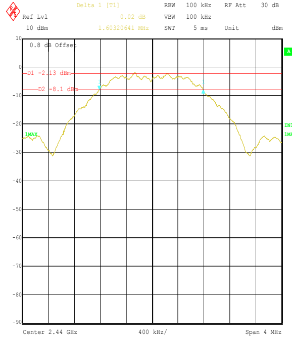
Title: Raymarine 46813JD10 EUT S100 Controller FCC P15.247 Comment A: 6 dB Bandwidth Middle Channel Date: 4.JAN.2005 14:14:43
