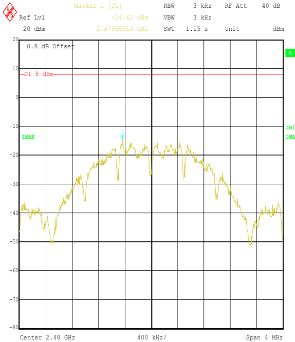
Title: Raymarine 46813JD10 EUT S100 Controller FCC P15.247 Comment A: Peak Power Spectral Density Top Channel Date: 4.JAN.2005 14:35:21
