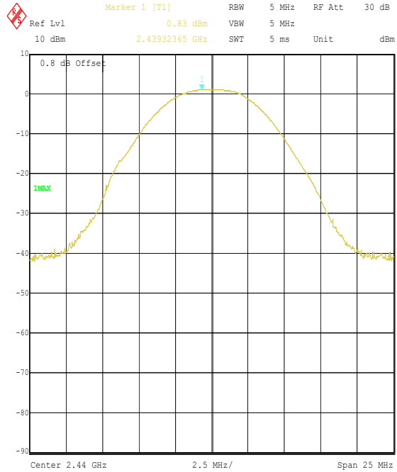
Title: Raymarine 46813JD10 EUT S100 Controller FCC P15.247 Comment A: Peak Output Power Middle Channel Date: 4.JAN.2005 14:37:53
