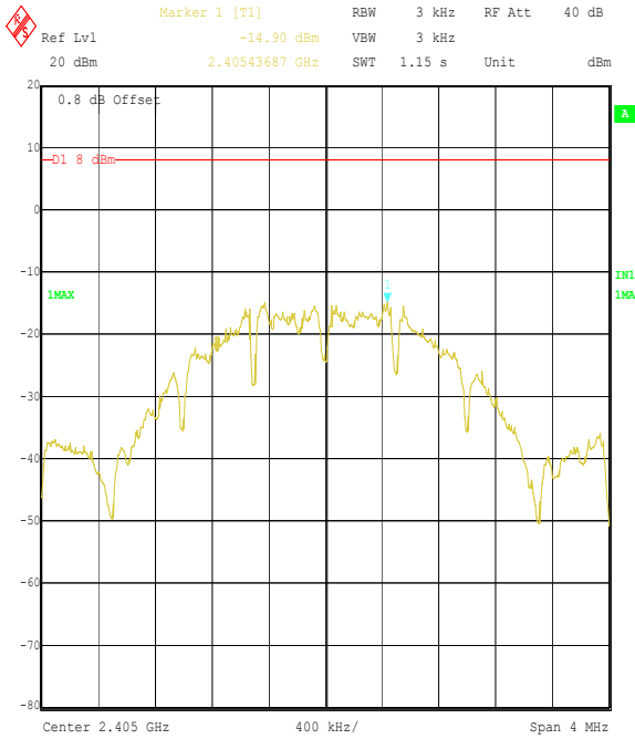
Title: Raymarine 46813JD10 EUT S100 Controller FCC P15.247 Comment A: Peak Power Spectral Density Bottom Channel Date: 4.JAN.2005 14:33:08
