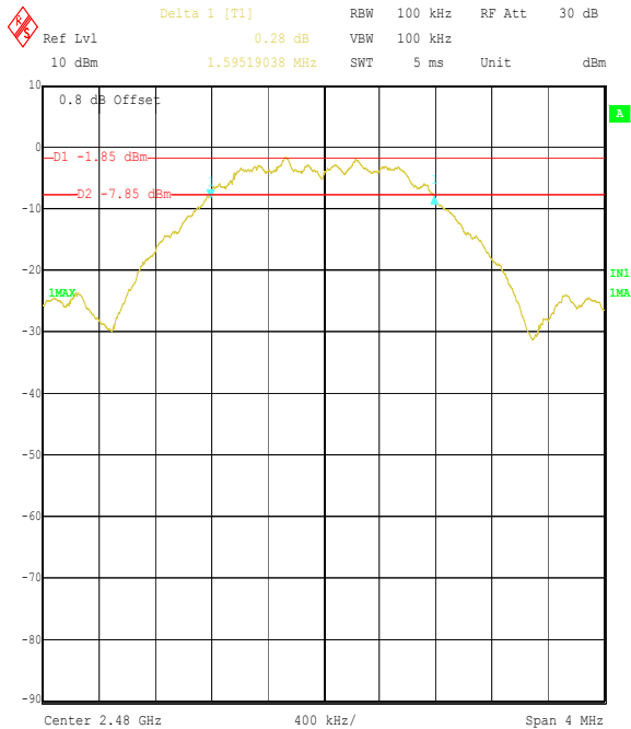
Title: Raymarine 46813JD10 EUT S100 Controller FCC P15.247 Comment A: 6 dB Bandwidth Top Channel Date: 4.JAN.2005 14:18:57
