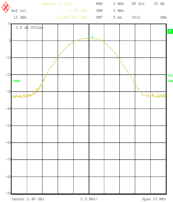
Title: Raymarine 46813JD10 EUT S100 Controller FCC P15.247 Comment A: Peak Output Power Top Channel Date: 4.JAN.2005 14:37:01
