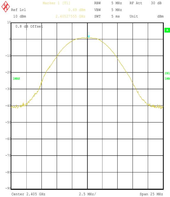
Title: Raymarine 46813JD10 EUT S100 Controller FCC P15.247 Comment A: Peak Output Power Bottom Channel Date: 4.JAN.2005 14:38:51
