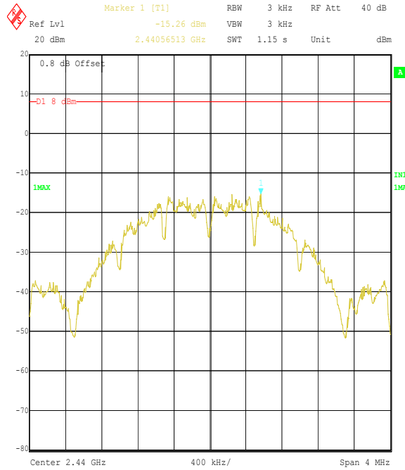
Title: Raymarine 46813JD10 EUT S100 Controller FCC P15.247 Comment A: Peak Power Spectral Density Middle Channel Date: 4.JAN.2005 14:34:23
