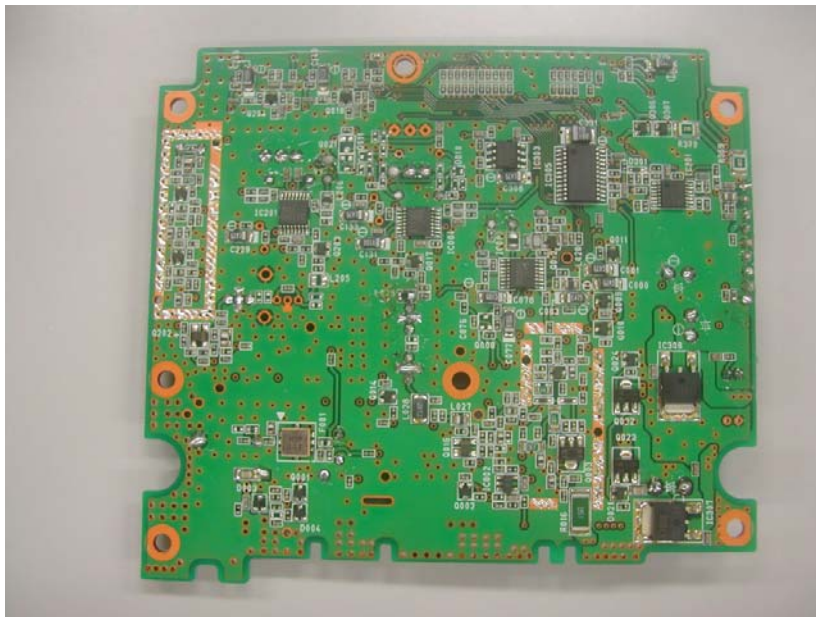
Ray49 RF/AF PCB - Front
