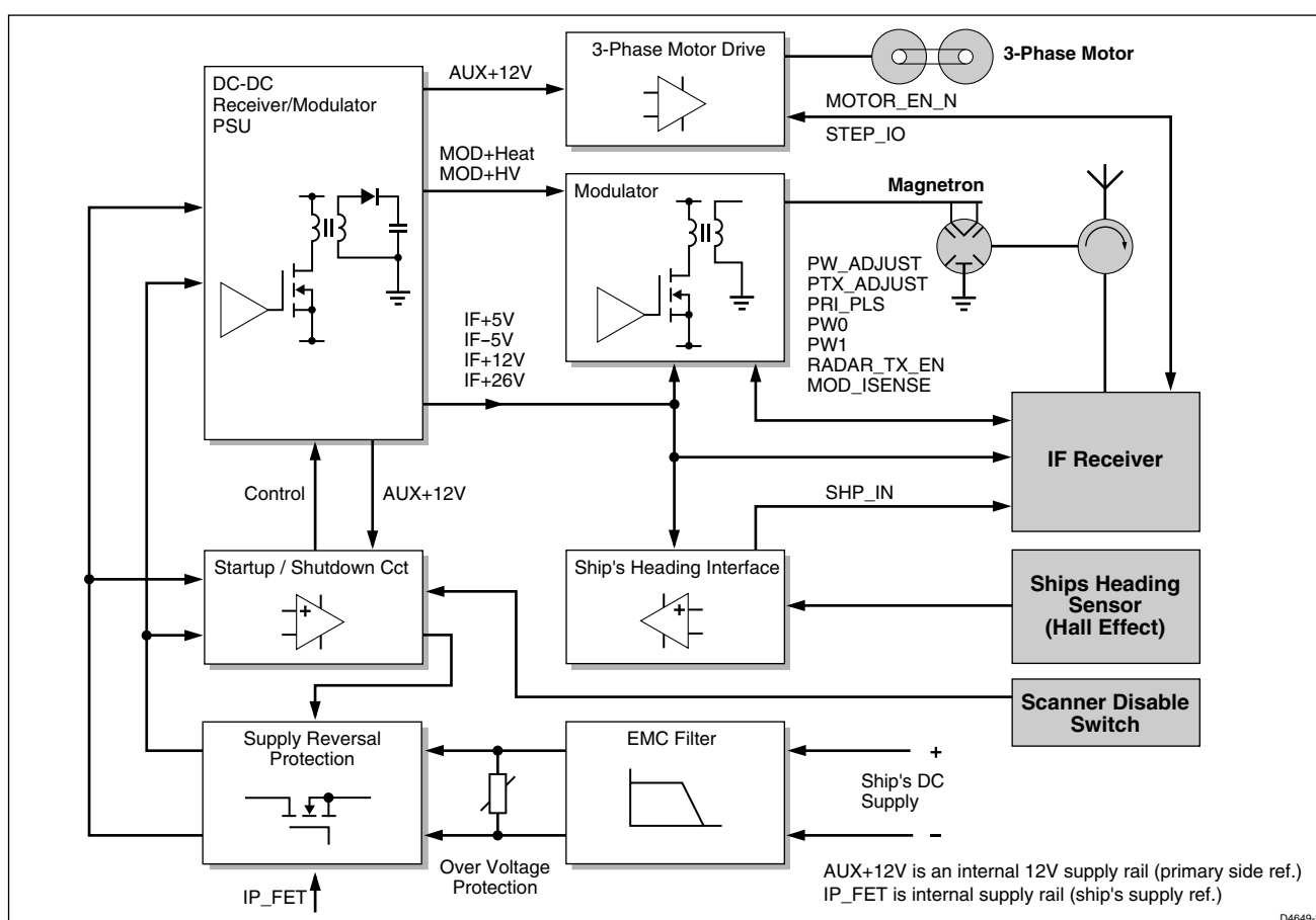
Figure 6. Modulator/PSU Overview
