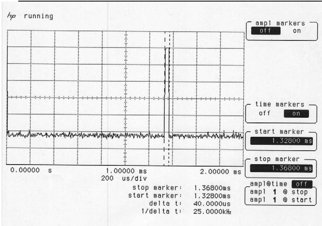
Graph PRF/555/1001/01
