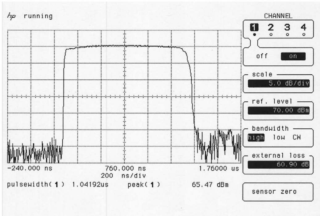
Graph PW/555/1001/08
