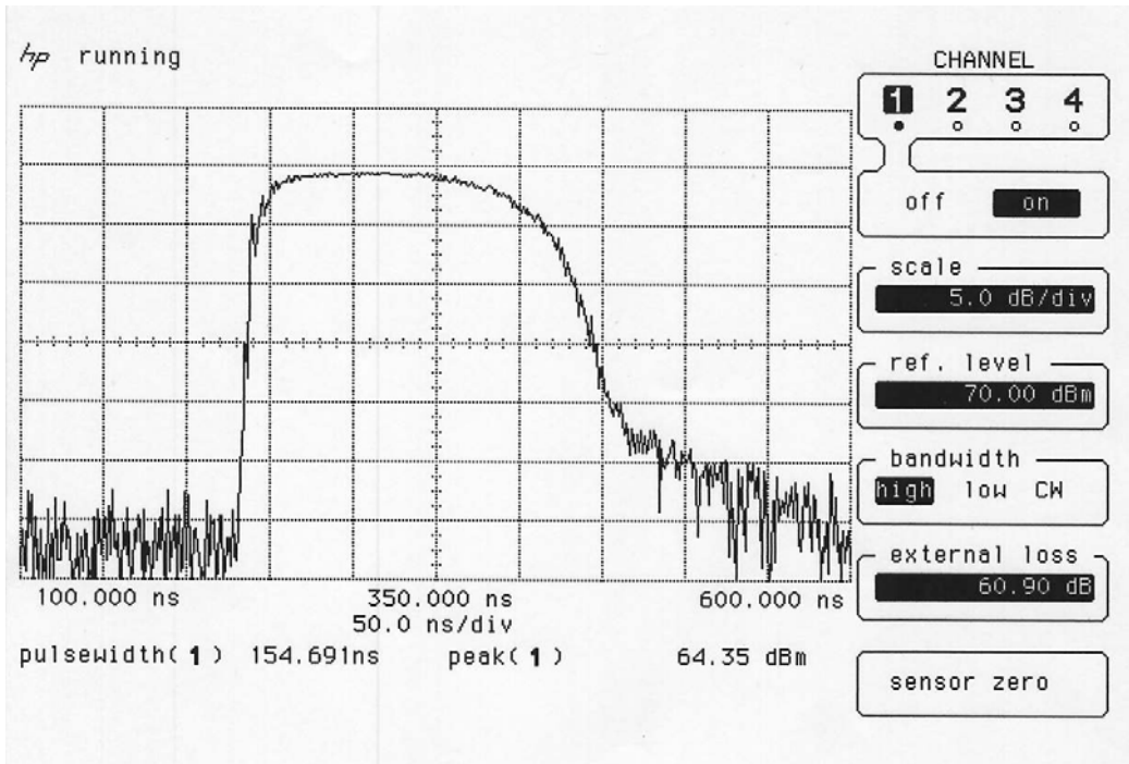
Graph PW/555/1001/03
