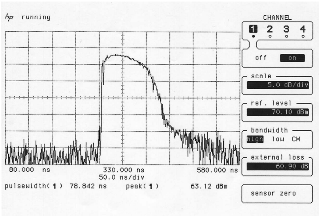
Graph PW/555/1001/01
