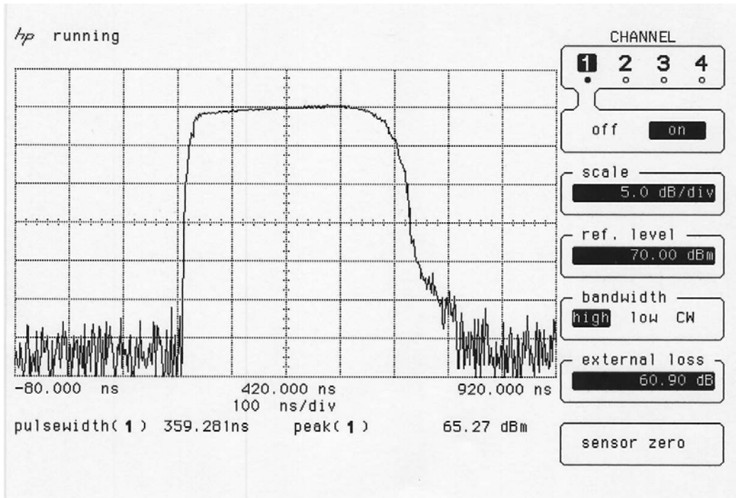
Graph PW/555/1001/05
