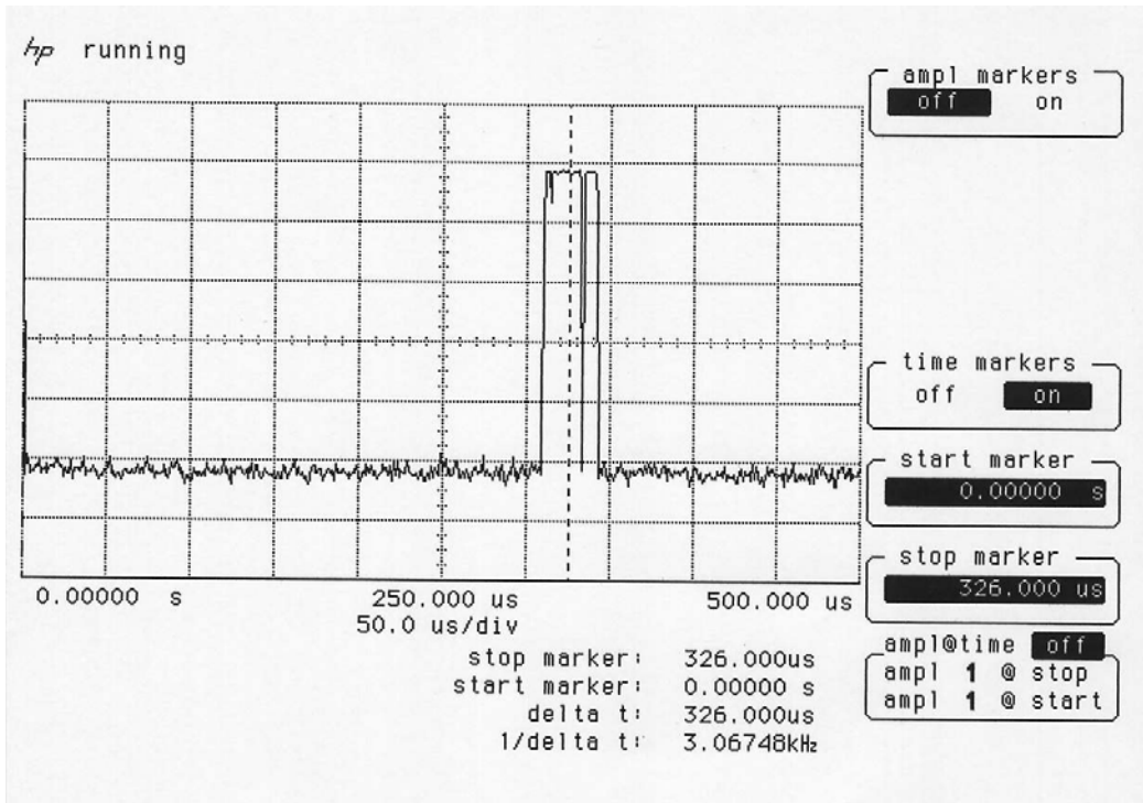
Graph PRF/555/1001/10
