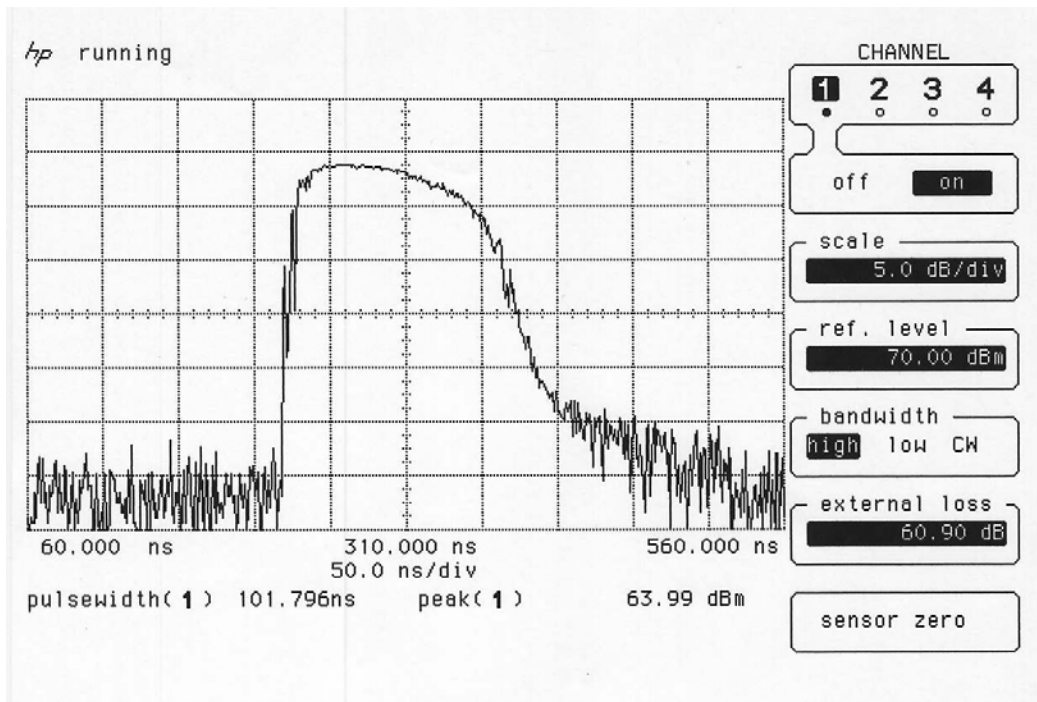
Graph PW/555/1001/02
