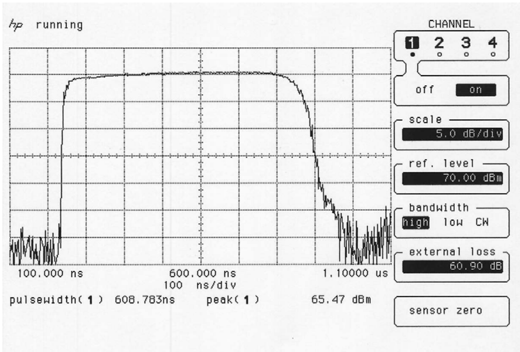
Graph PW/555/1001/07
