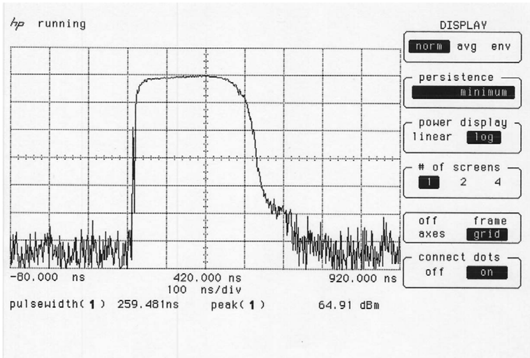
Graph PW/555/1001/04
