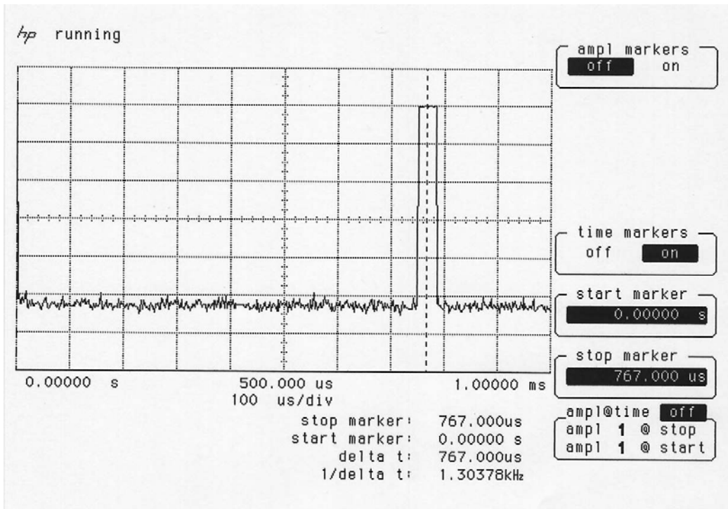
Graph PRF/555/1001/04
