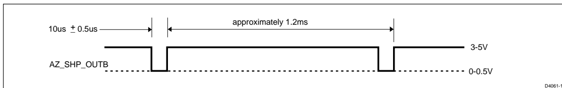
Figure 8: AZ_SHP_OUTB/AZIM_DNEG
