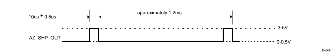
Figure 9: AZ_SHP_OUT/AZIM_DPOS
