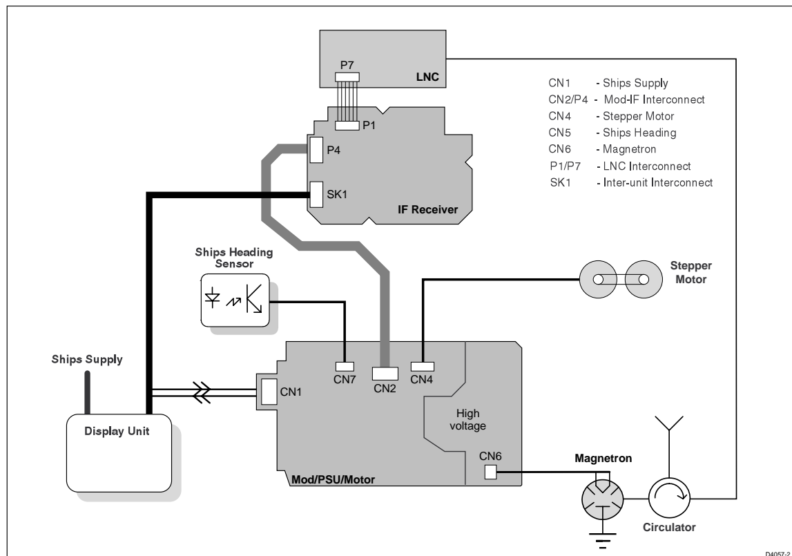
Figure 4: Scanner Interfaces
