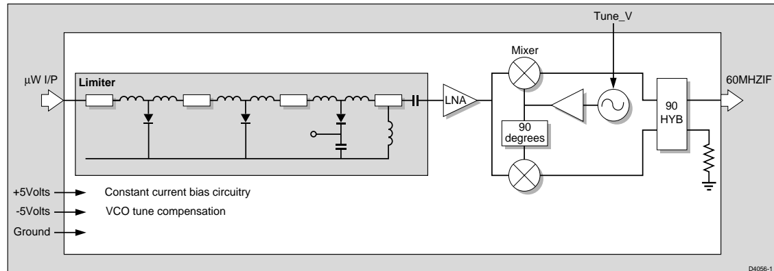
Figure 3: LNC Configuration
