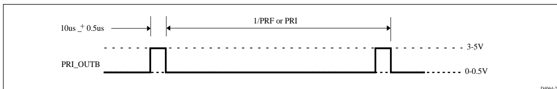
Figure 11: PRI_OUTB/PRI_DNEG
