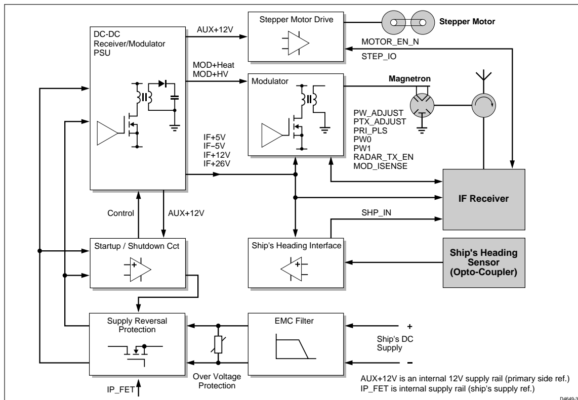
Figure 6: Modulator/PSU Overview
