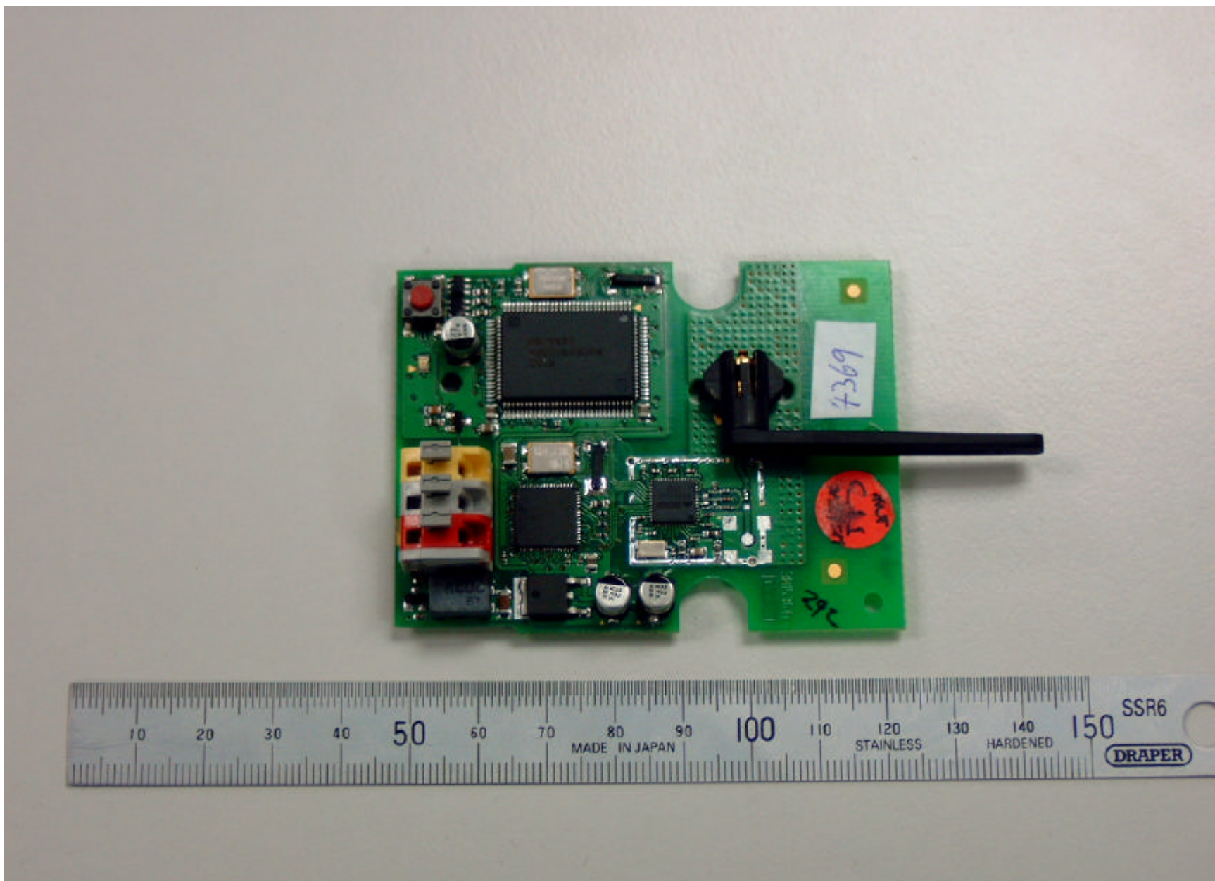
Basestation
