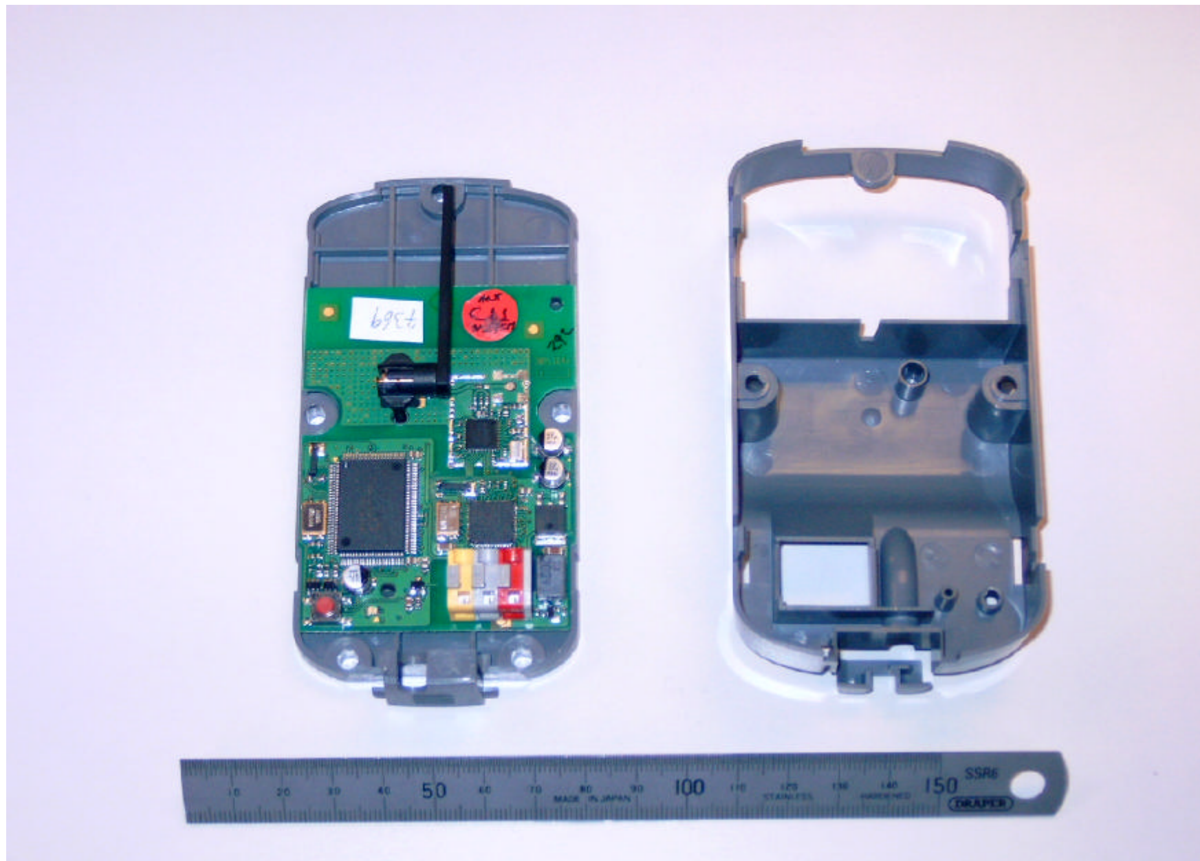
Basestation
