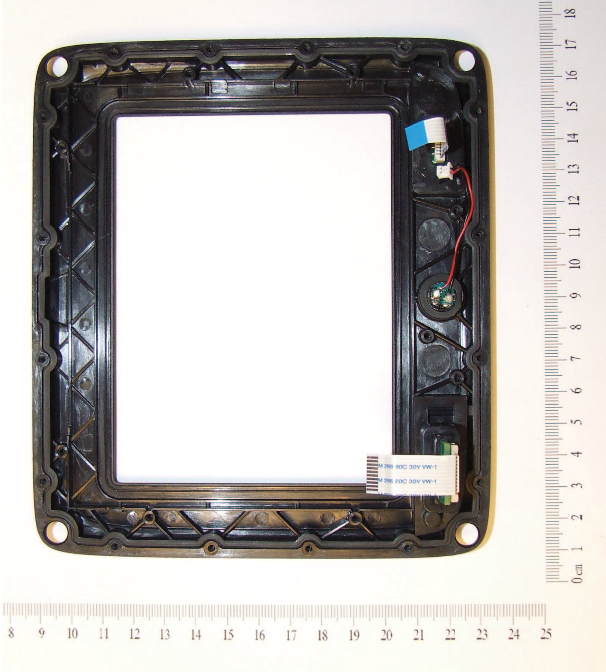
Figure 14 - Rear of front fascia
