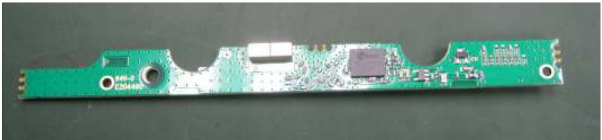
GPS Board Top
