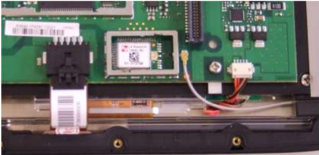
Close up of RF module and antenna connection
