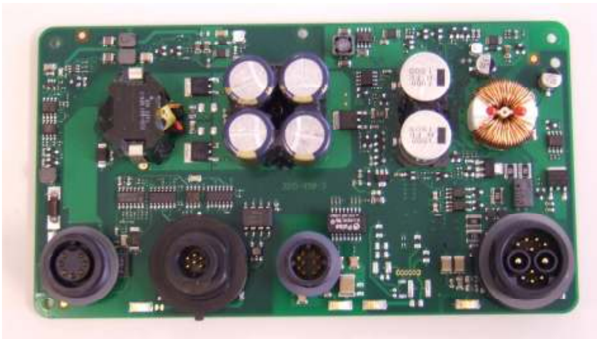
Connector side of I/O board (Fishfinder version)
