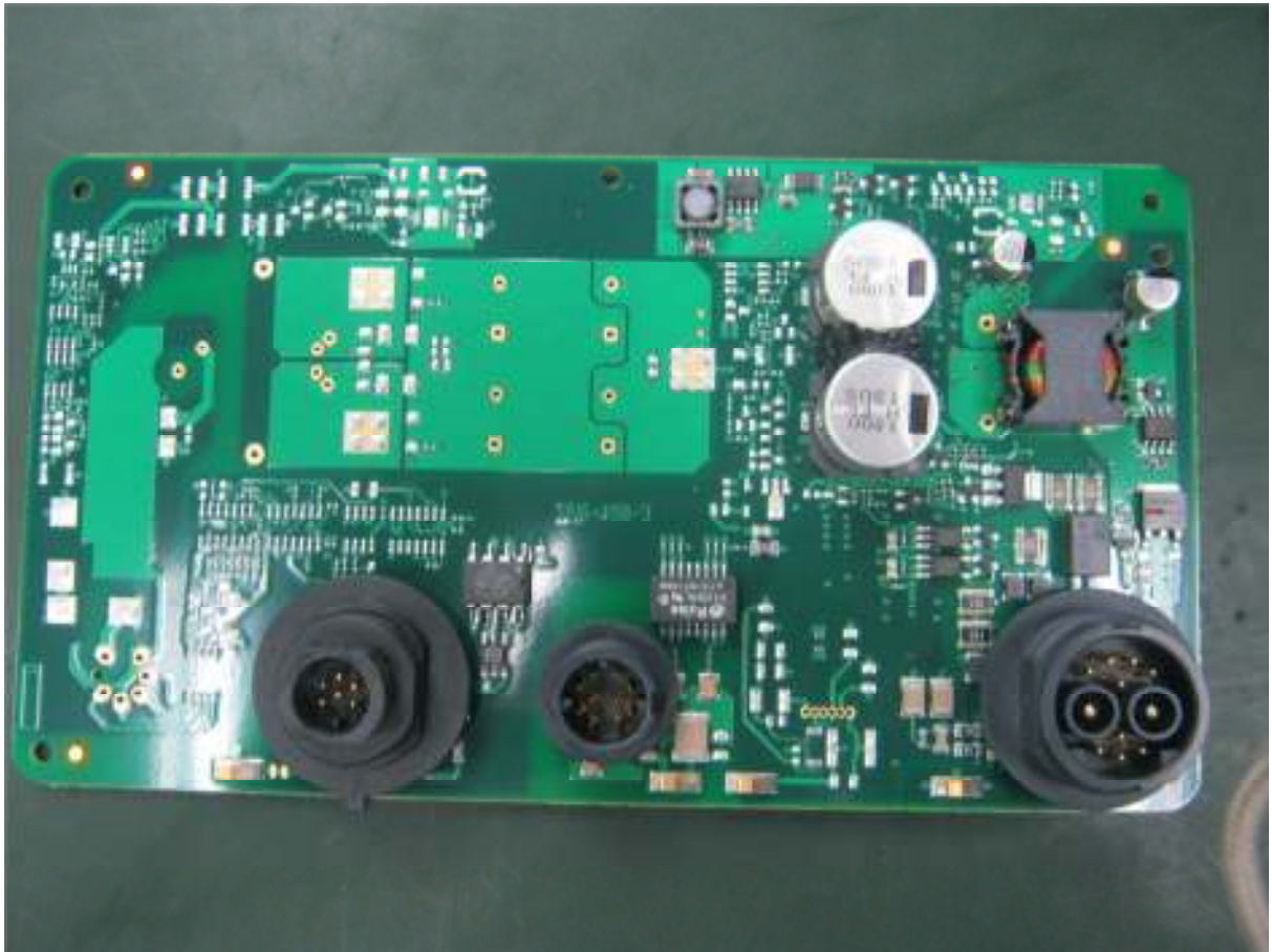
Connector side of I/O board (non-fishfinder version)
