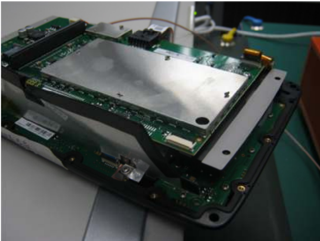
Top view of LCD and CPU module
