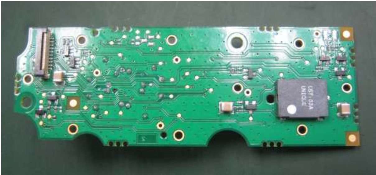
Keyboard PCB Back
