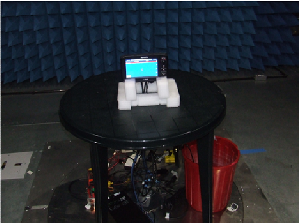
15.247 setup
