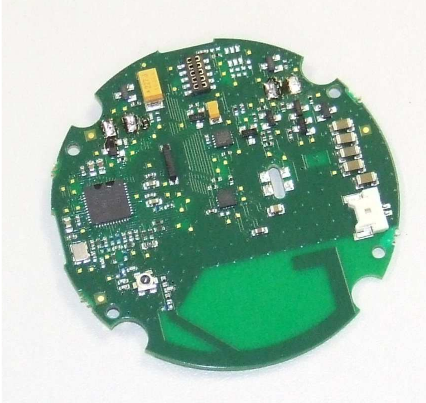
Figure 2 – Top of PCB
