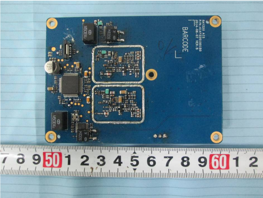
EUT –Base AIS Board Top View
