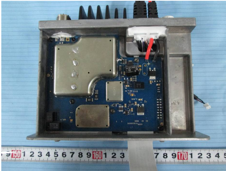
EUT – Base Cover off View 5
