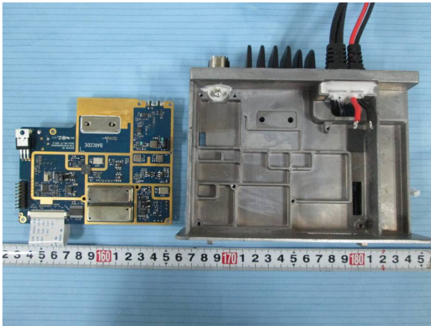
EUT – Base Cover off View 7
