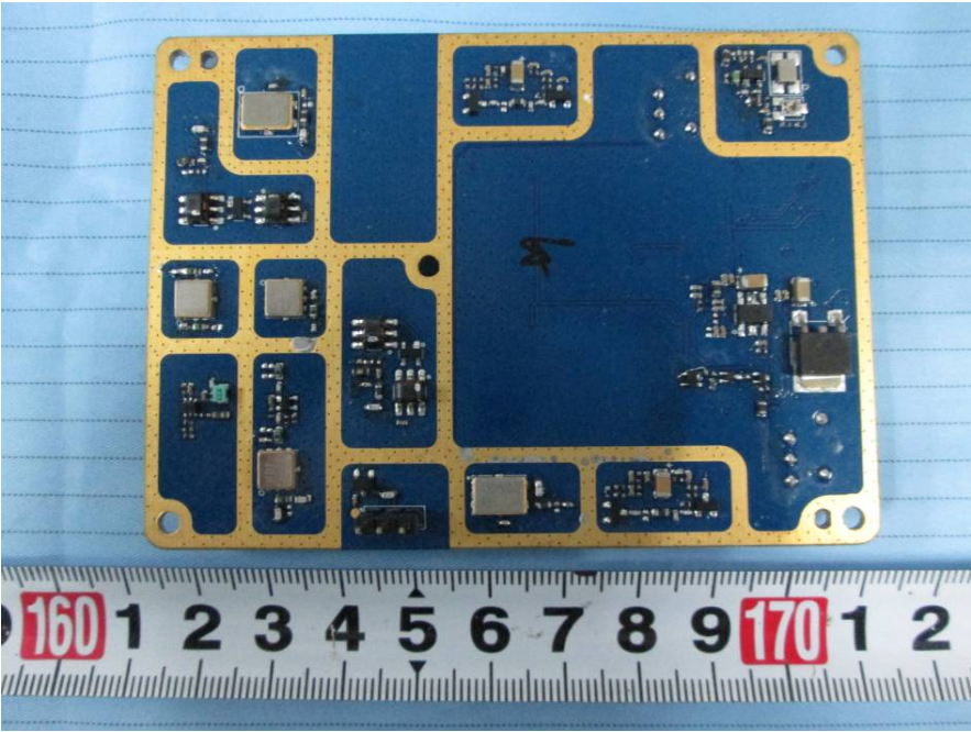
EUT –Base AIS Board Bottom View
