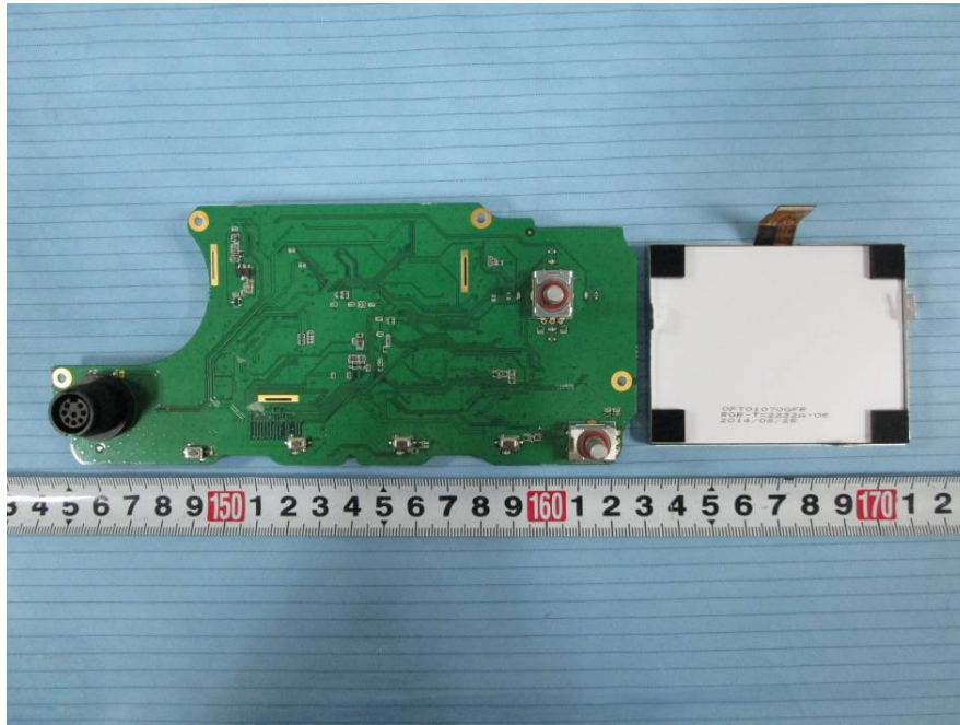
EUT –Base LCD Screen off View
