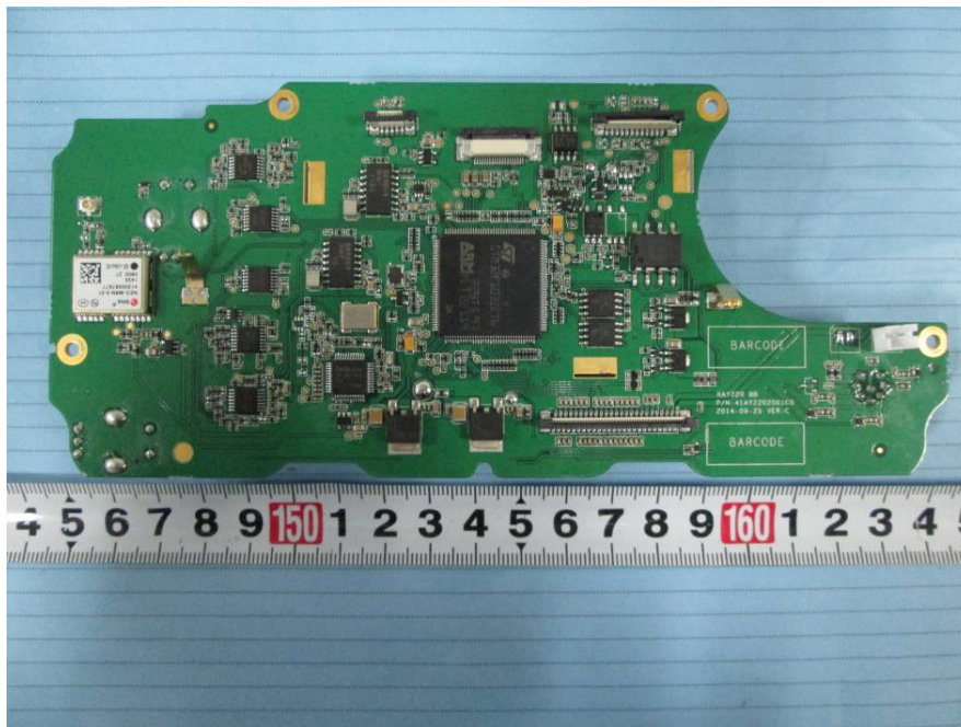
EUT –Base Control Board Bottom View
