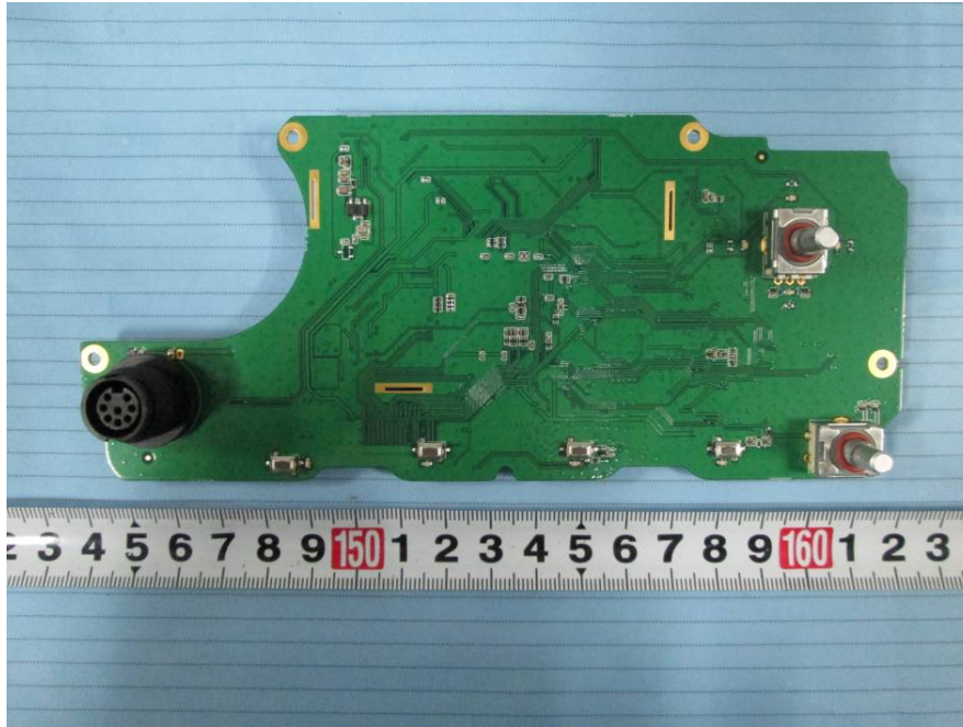
EUT –Base Control Board Top View
