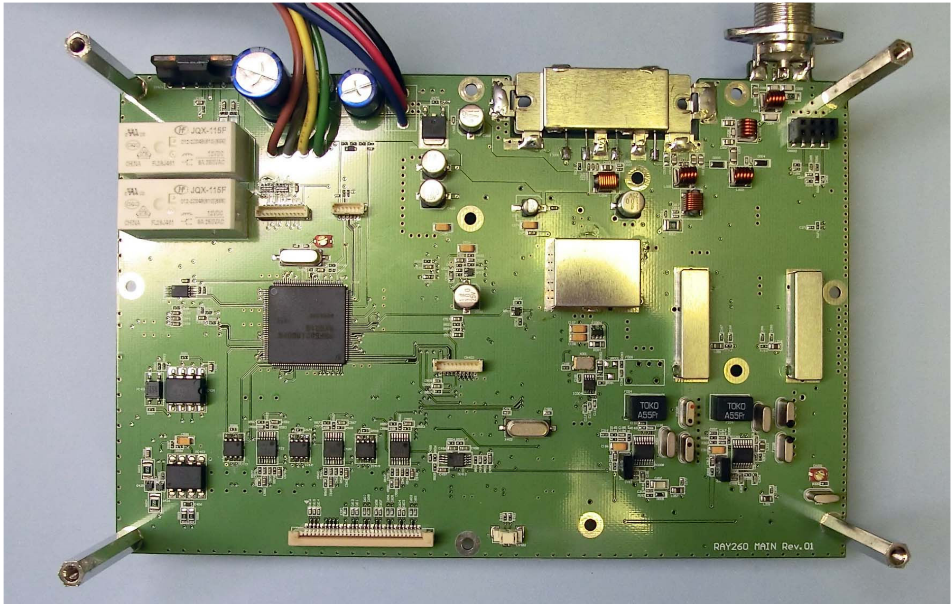
Figure 1 – Main PCB – Top
