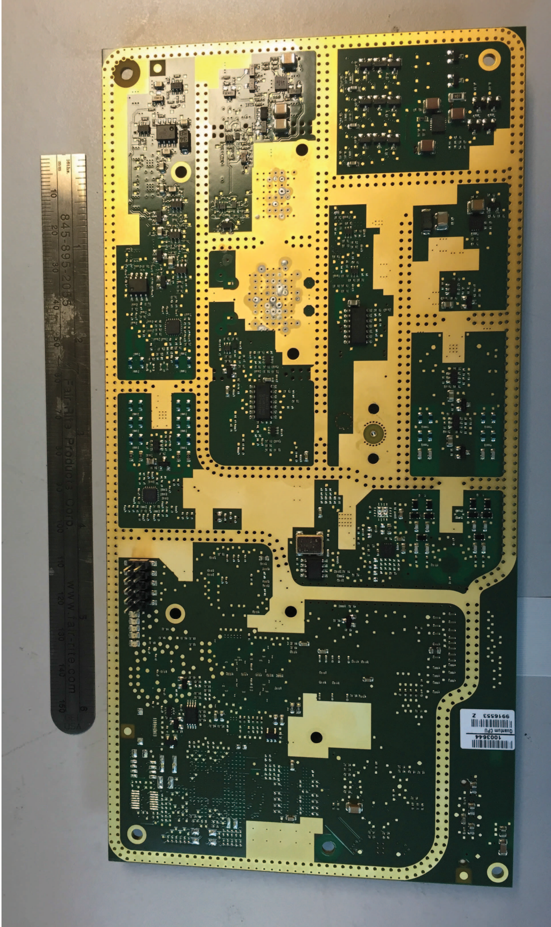
Figure 8 – RF PCB – Back
