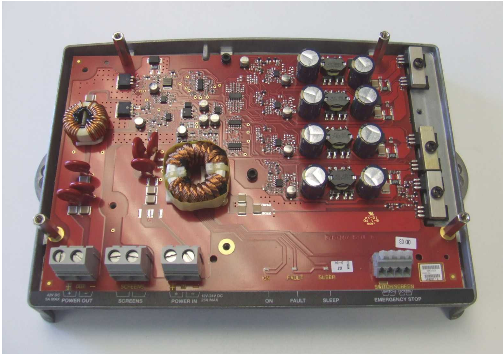
VCM100 - with front cover and connector cover removed
