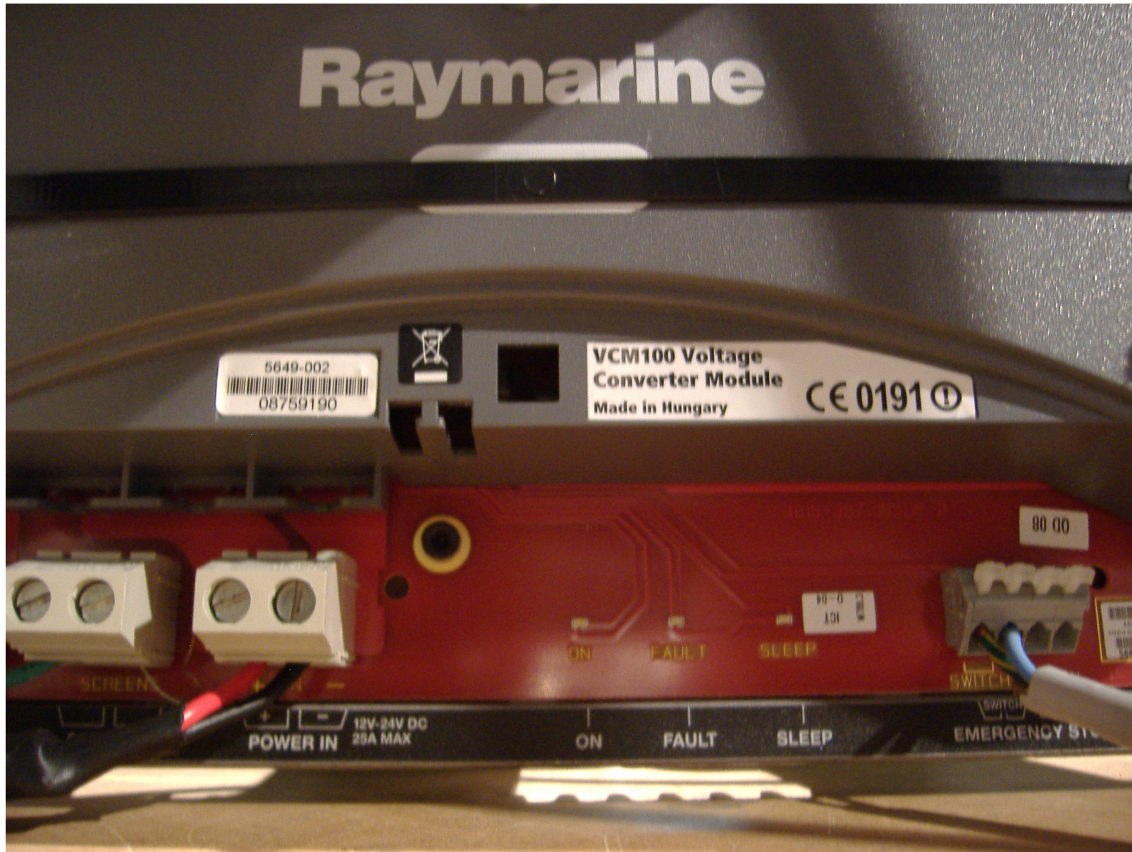
VCM100 labels. Left-hand label identifies product by part number and serial number. 5649-002 will be replaced by E52091 on production units.
