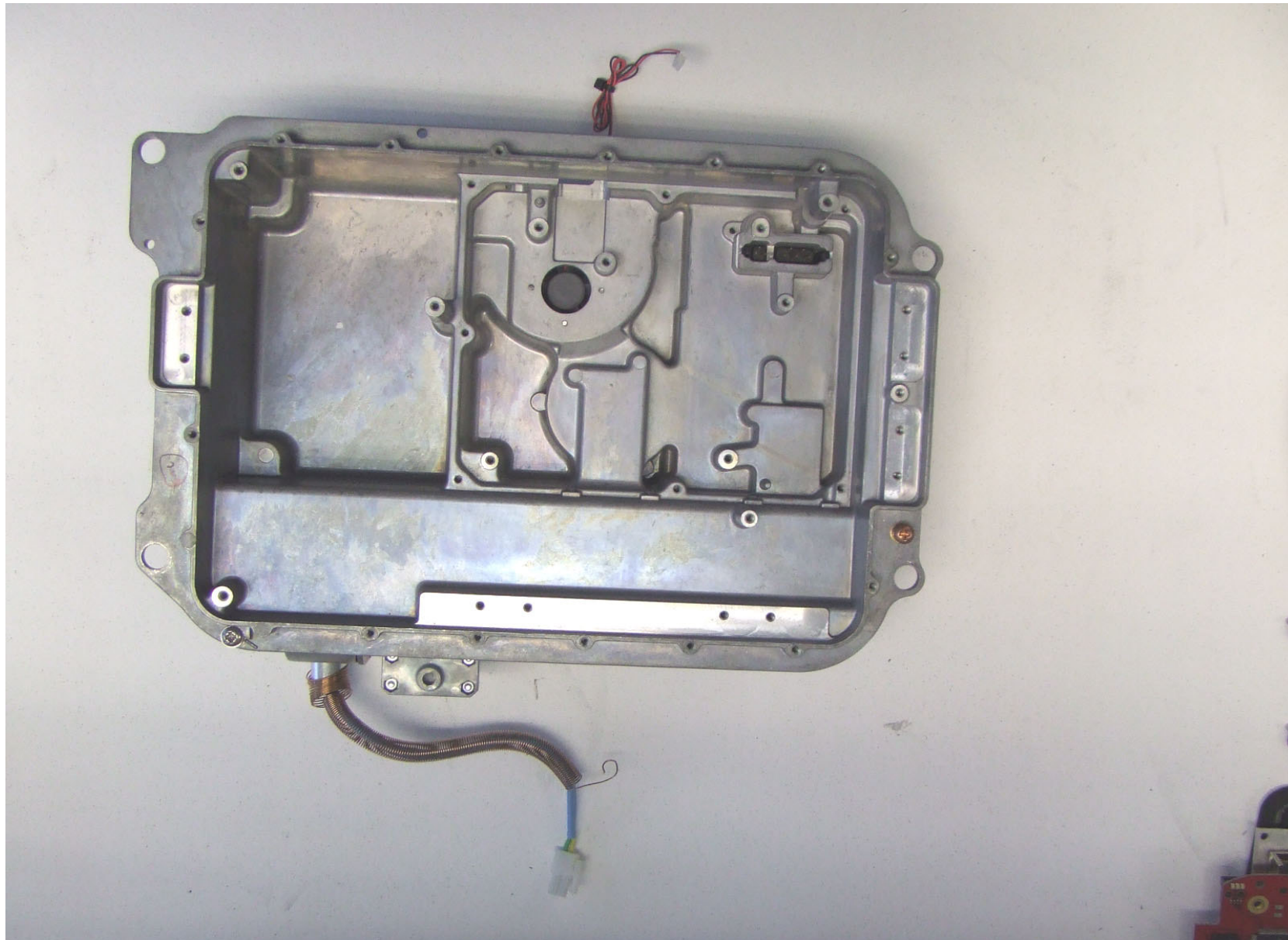
NGS 12kW Digital Open Array Radar Scanner - core module bottom view with modulator/psu pcb and IF assembly removed.
