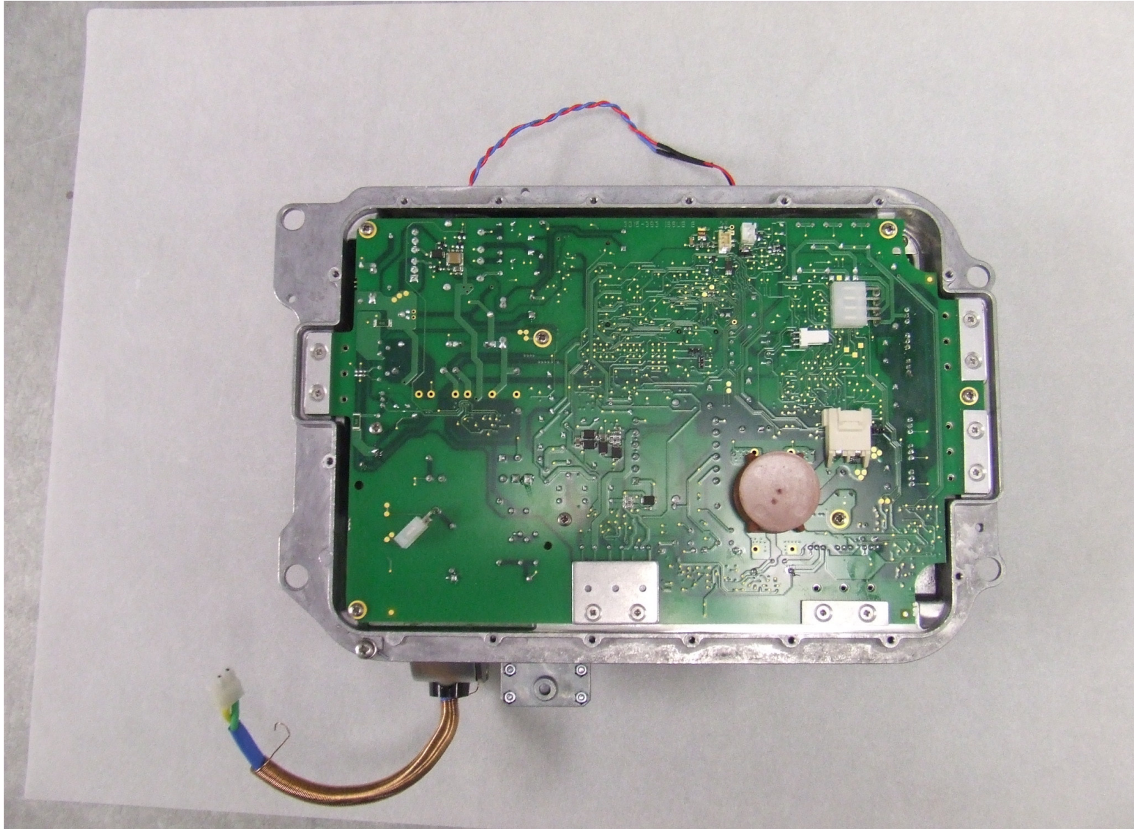
NGS 12kW Digital Open Array Radar Scanner - core module bottom view with cover removed to show underside of modulator/psu pcb - magnetron and cooling fan disconnected.
