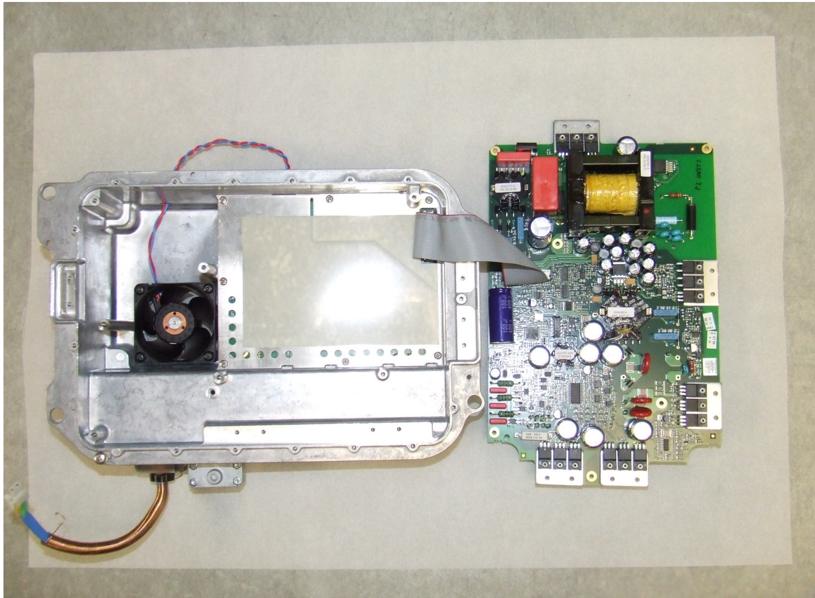
NGS 12kW Digital Open Array Radar Scanner - core module bottom view with modulator/psu pcb removed to show IF assembly screening cover.
