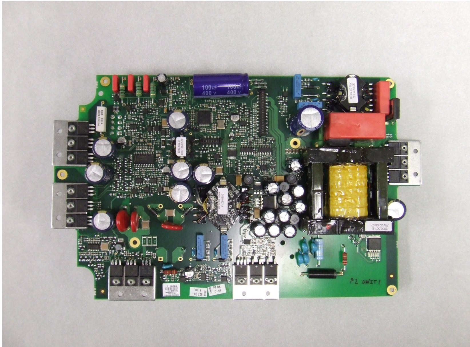
NGS 12kW Digital Open Array Radar Scanner - modulator/psu pcb top view.
