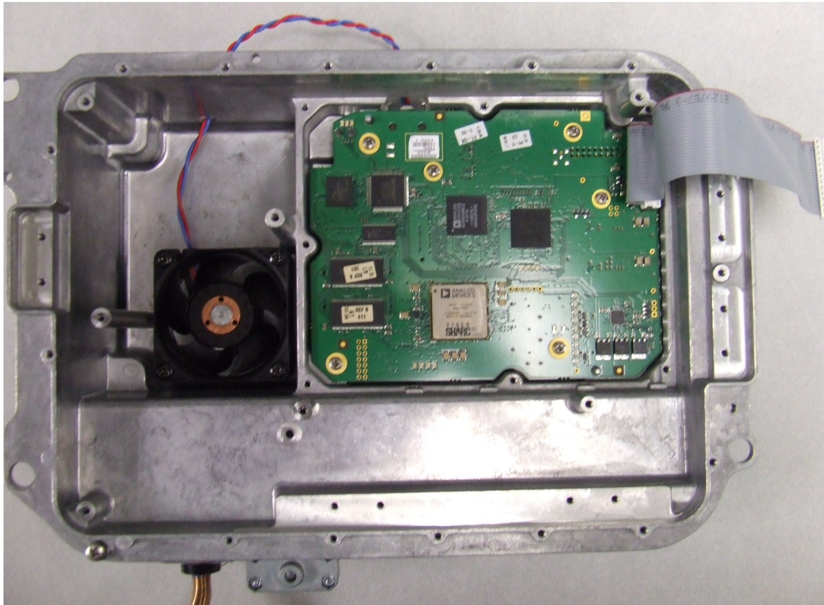
NGS 12kW Digital Open Array Radar Scanner - core module bottom view with modulator/psu pcb and IF assembly cover removed.
