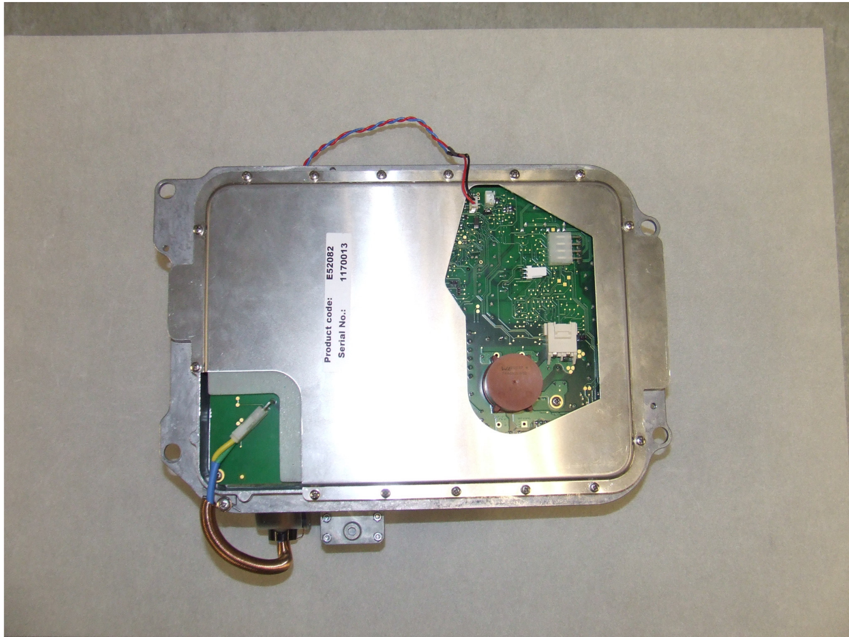
NGS 12kW Digital Open Array Radar Scanner - core module bottom view with magnetron and cooling fan connected. Interior view 11
