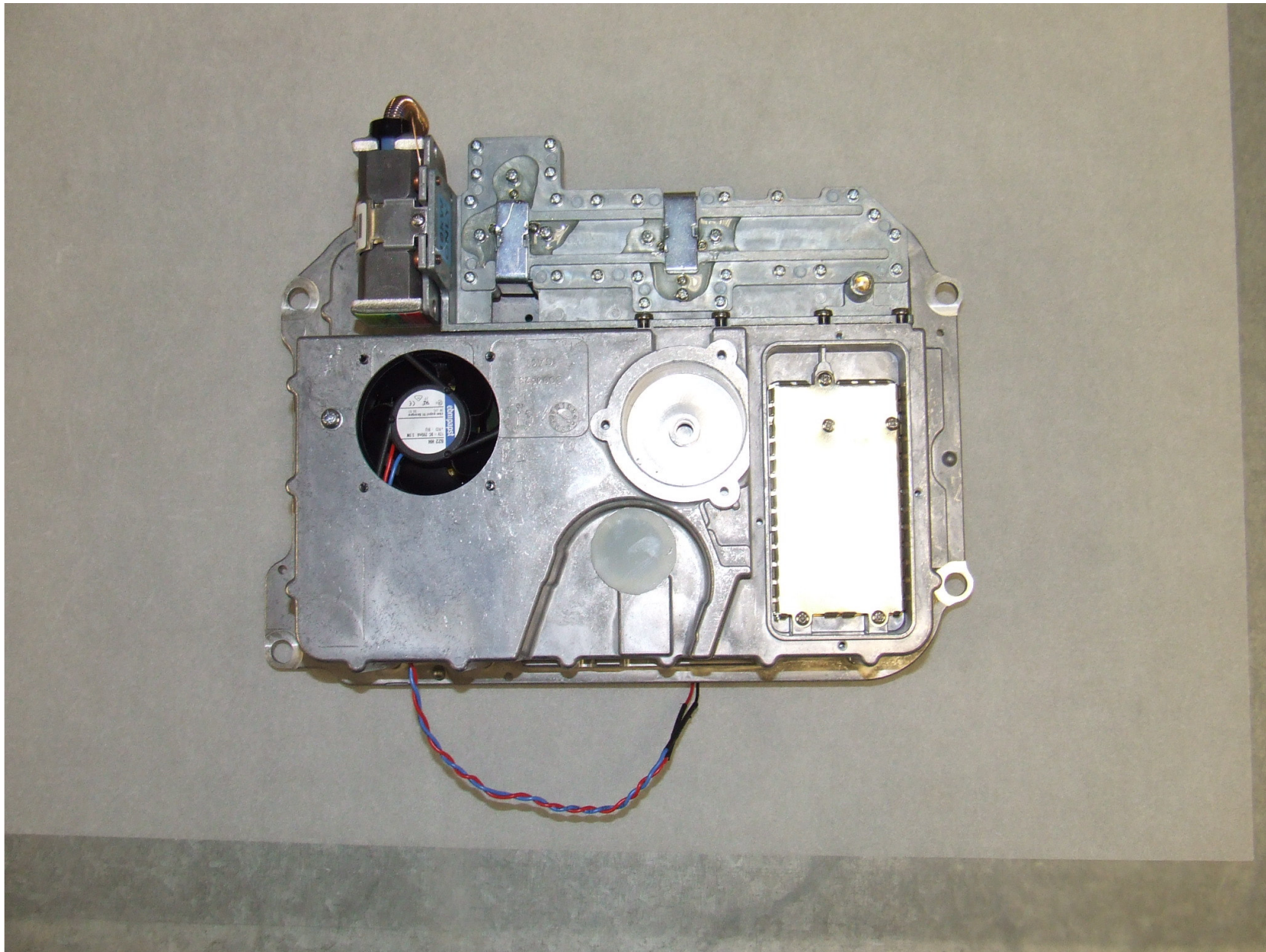
NGS 12kW Digital Open Array Radar Scanner - core module top view with cover removed to show LNC assembly.
