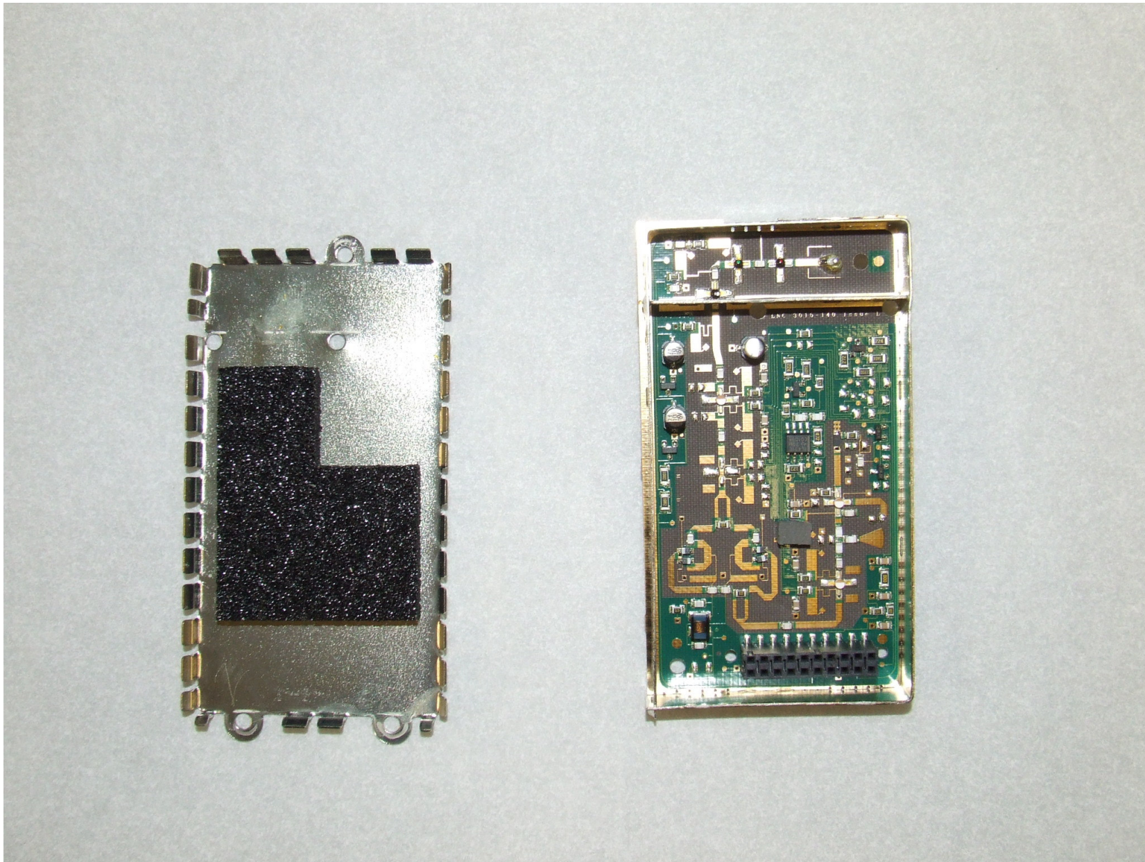
NGS 12kW Digital Open Array Radar Scanner - LNC assembly with screening can removed.
