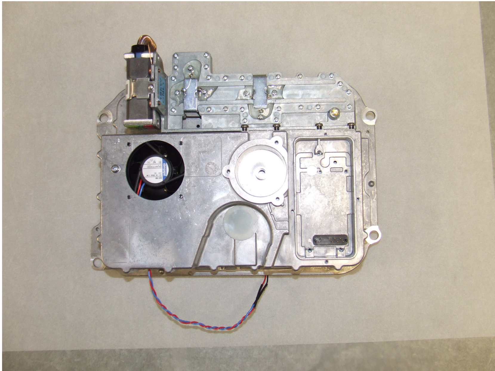
NGS 12kW Digital Open Array Radar Scanner - core module top view with LNC assembly removed.
