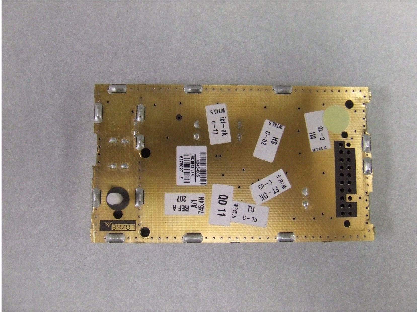
NGS 12kW Digital Open Array Radar Scanner - LNC assembly underside.
