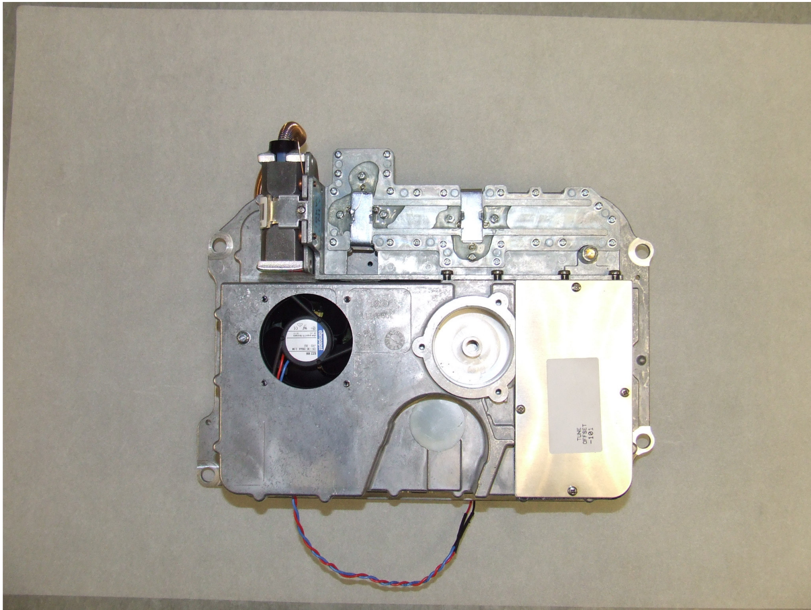
NGS 12kW Digital Open Array Radar Scanner - core module top view showing magnetron, circulator, cooling fan and fixed/rotary joint coupling. Interior view 6
