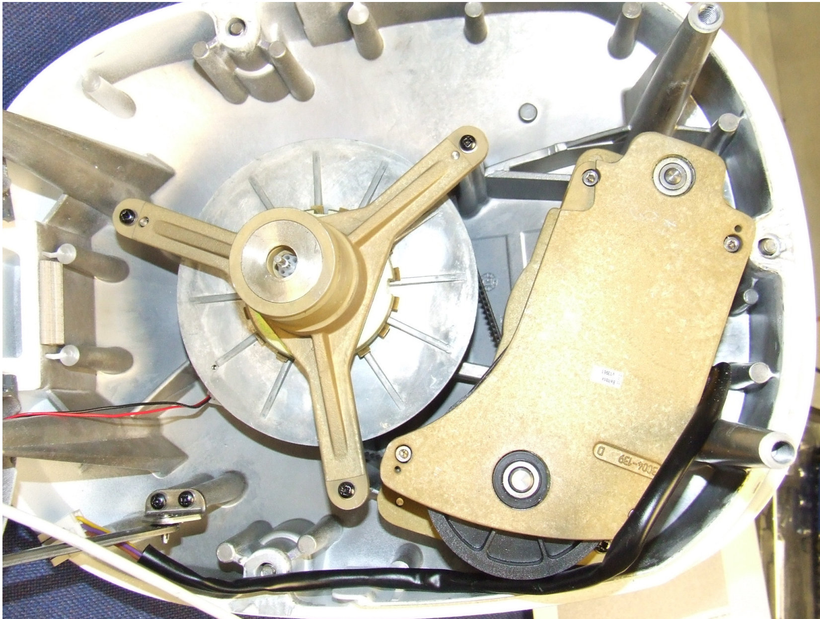
NGS 12kW Digital Open Array Radar Scanner - view of motor/gearbox assembly and rotating joint.
