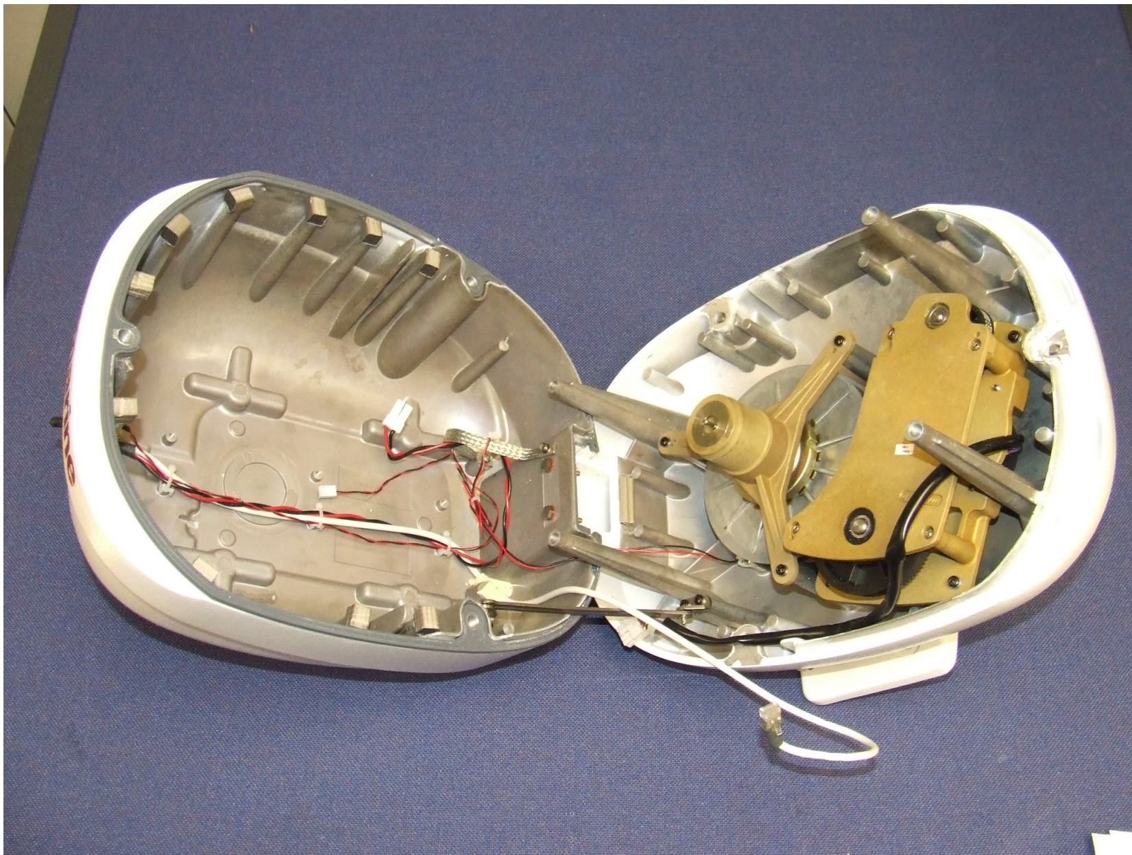
NGS 12kW Digital Open Array Radar Scanner - interior view with radar core removed.
