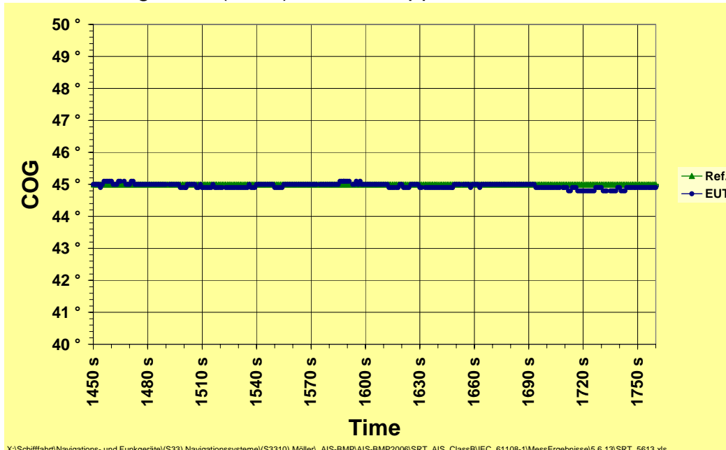
Course over ground (COG) vs. time, approx. 14.3Knots
