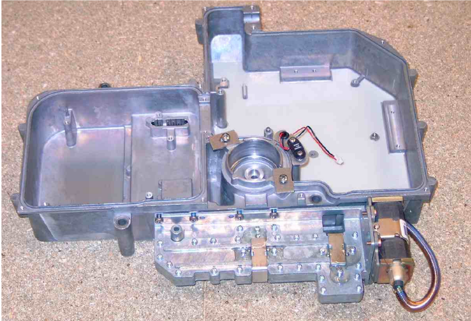
RD424 4kW 24" Radome Scanner
