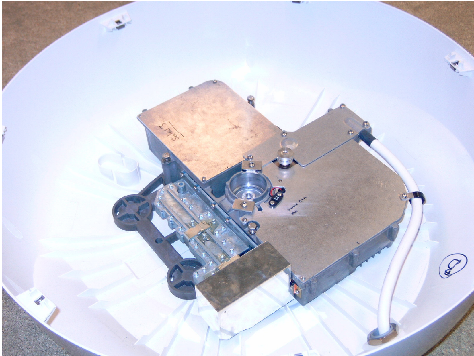
RD424 4kW 24" Radome Scanner Core with antenna removed. View showing circulator and magnetron screening box.
