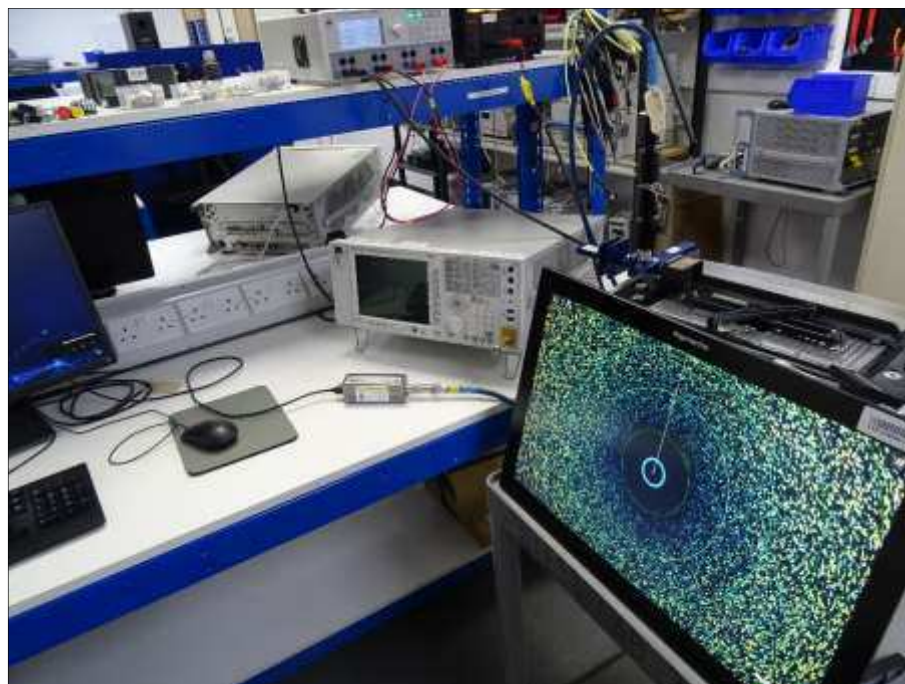
Figure 78 - Conducted Test Setup
