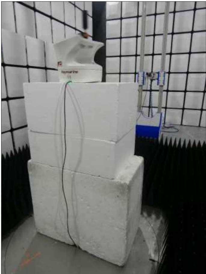
Figure 77 - Test Setup - 18 GHz to 40 GHz
