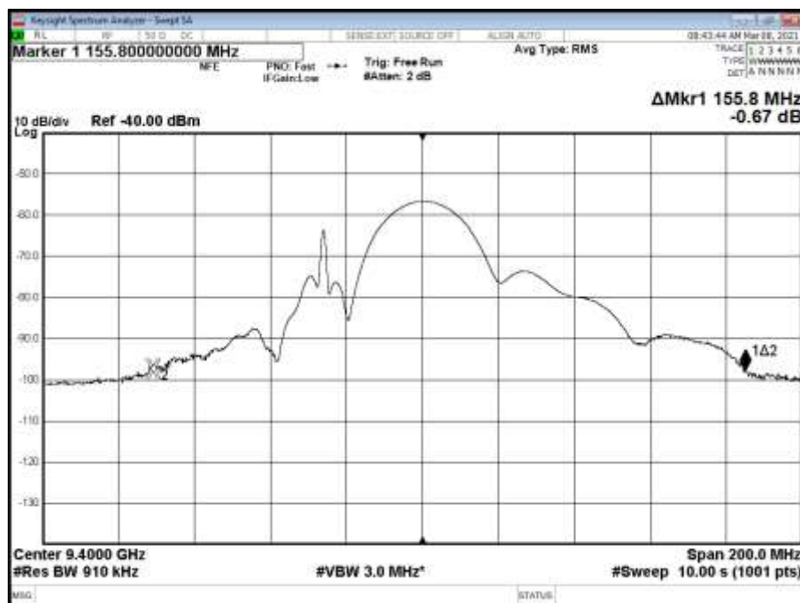
Figure 20 - 9400 MHz, CW, 46 ns, 40 dB Bandwidth
