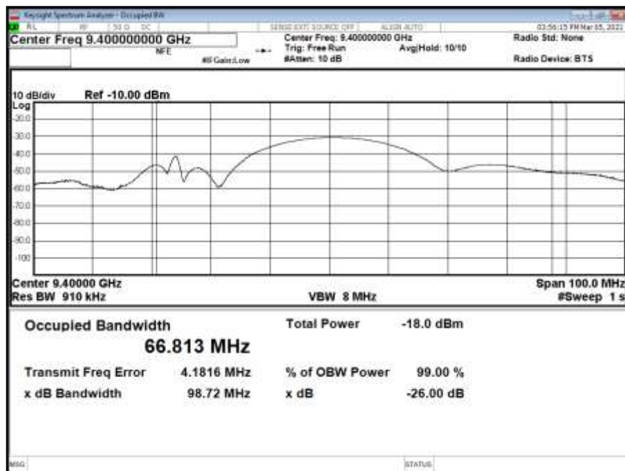
Figure 19 – 9400 MHz, CW, 46 ns, 99% Occupied Bandwidth
