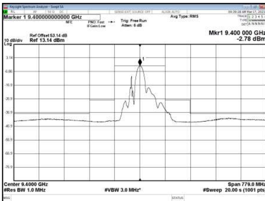
Figure 55 - 9400 MHz, CW, 46 ns (FCC Mask)
