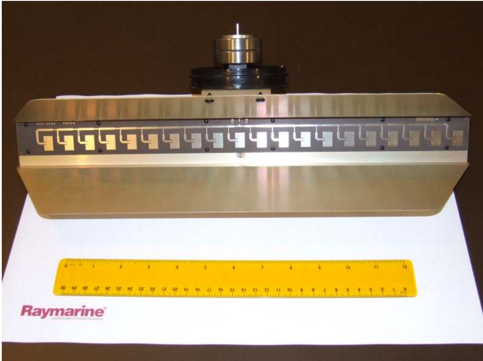
Figure 5 - RD418HD Antenna Front
