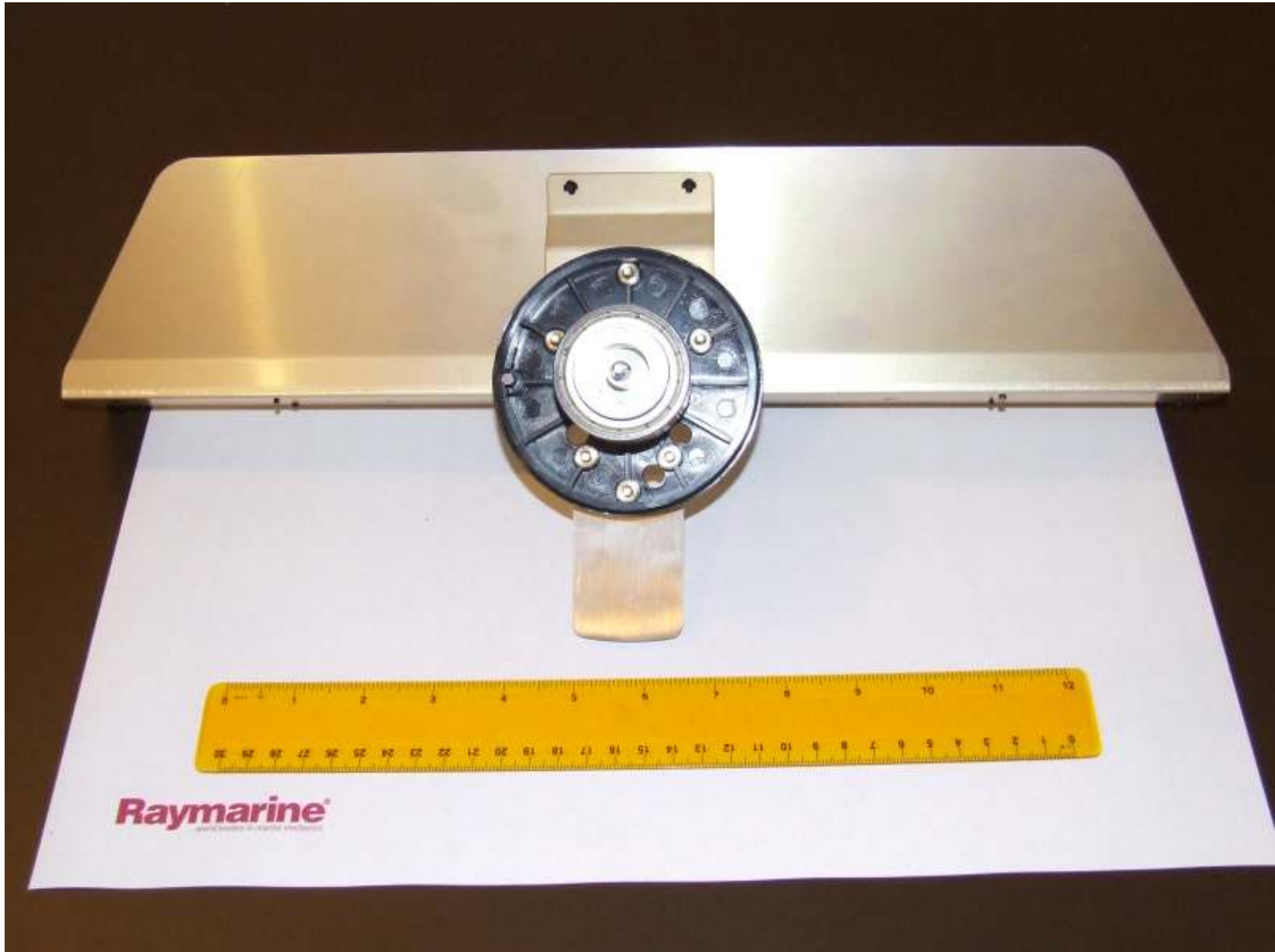
Figure 4 - RD418HD Antenna Base
