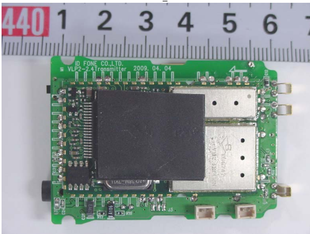
Main board_Bottom
