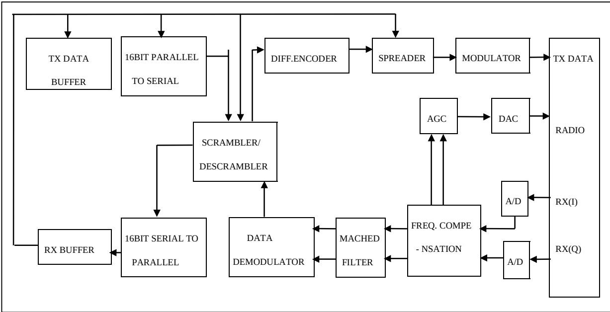
Spread Spectrum Engine Block Diagram
