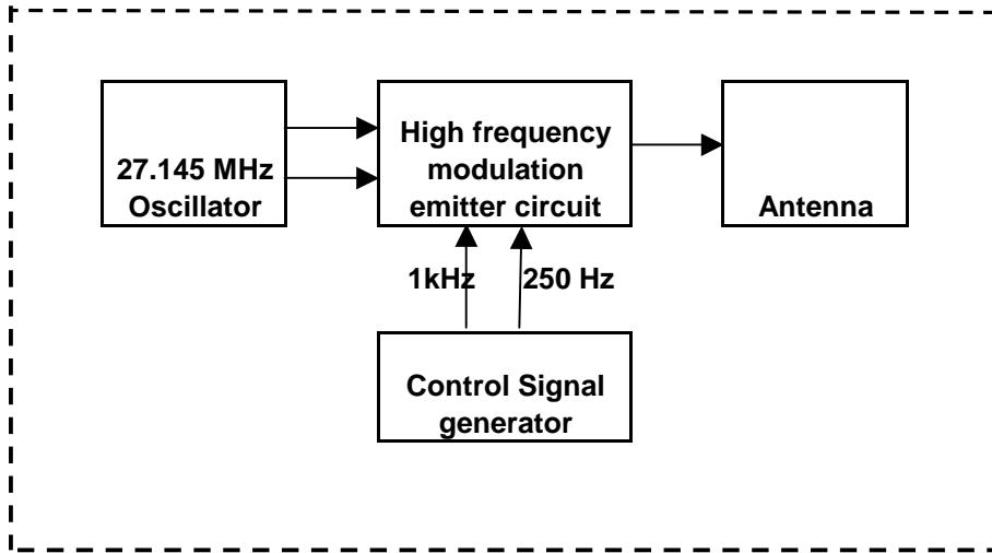
Transmitter circuit block diagram
