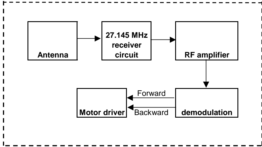
Receiver circuit block diagram
