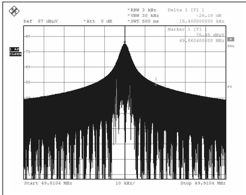
Bandwidth 1
