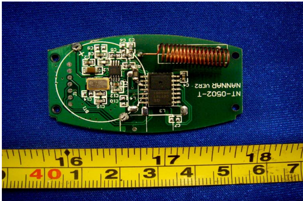
PCB-Front View
