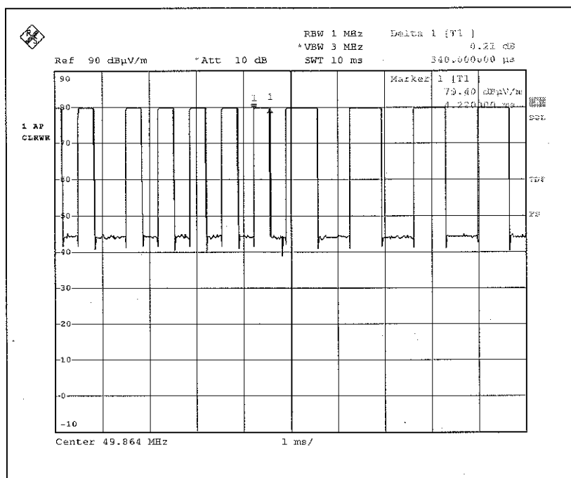
Duty Cycle 3
