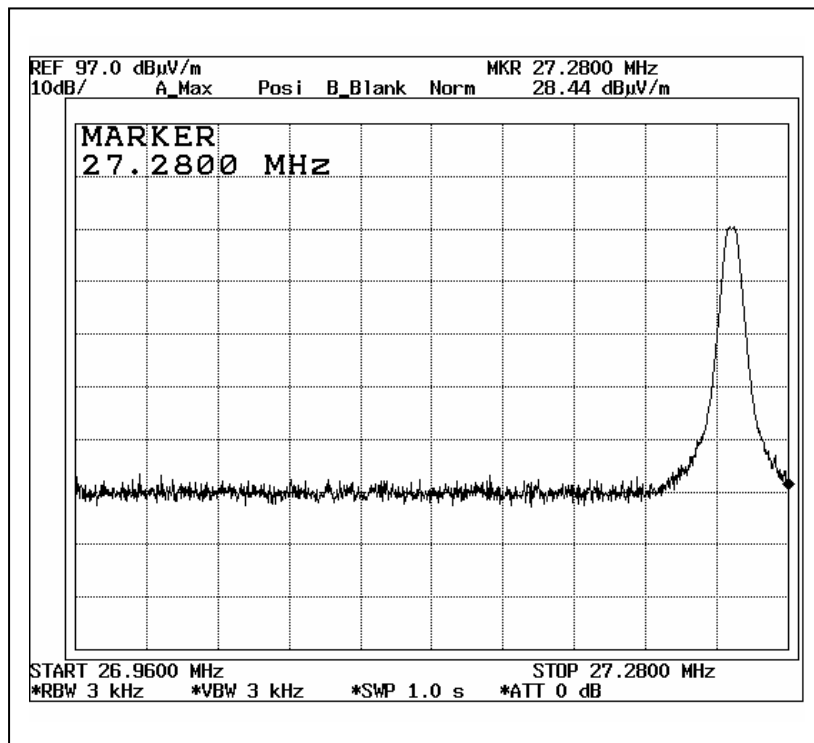
Bandwidth 2 (Channel 8)
