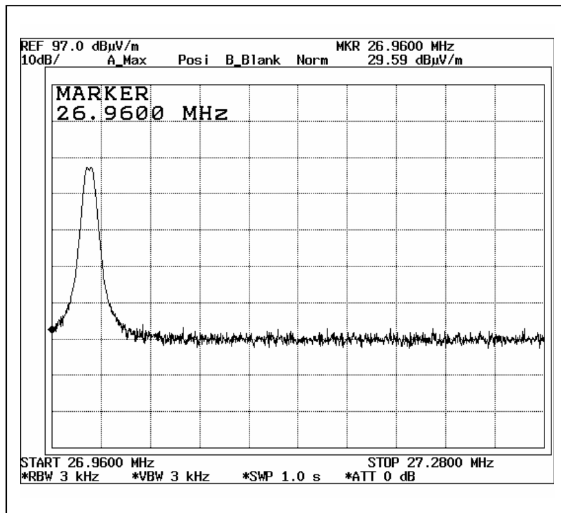
Bandwidth 1 (Channel 1)
