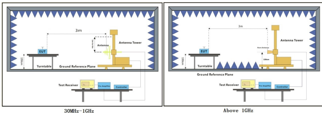
30MHz-1GHz
