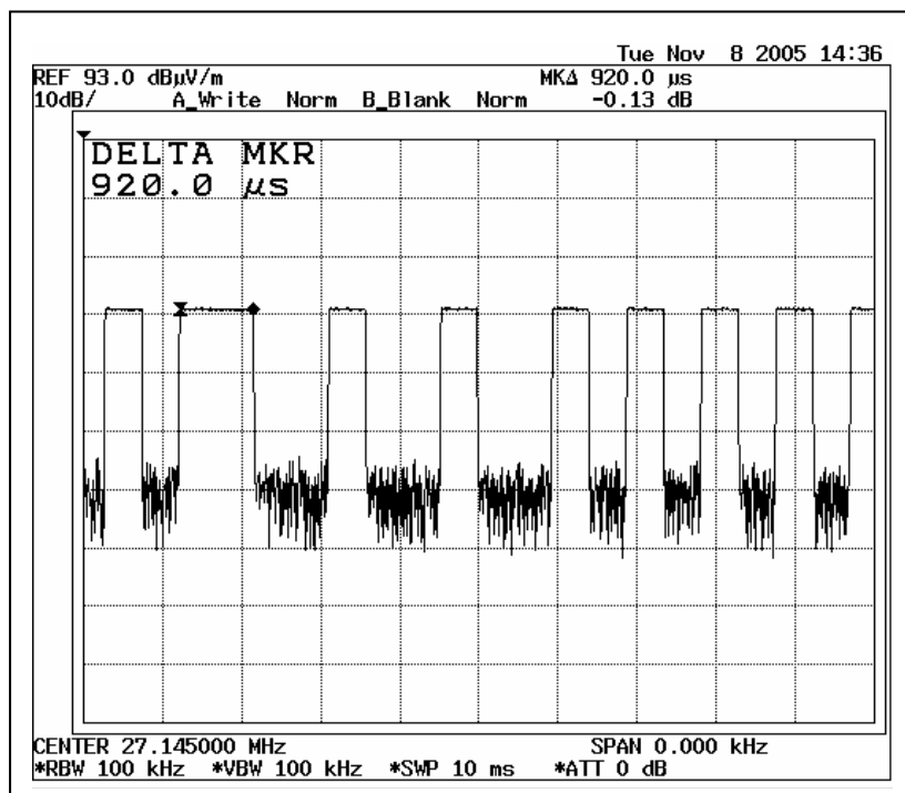
Duty Cycle 2
