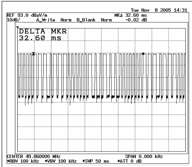
Duty Cycle 1
