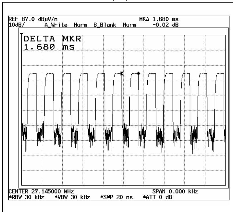
Duty Cycle
