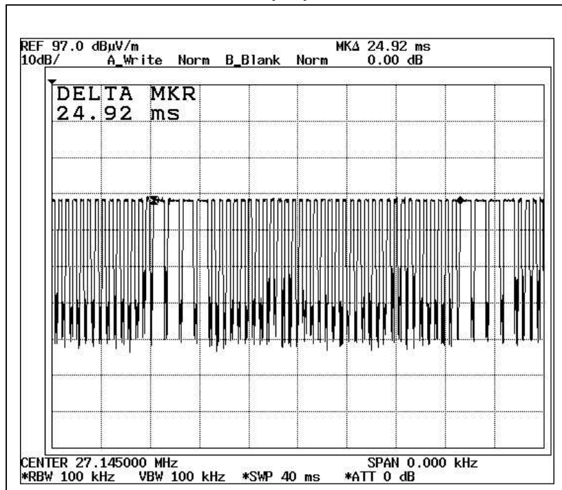
Duty Cycle
