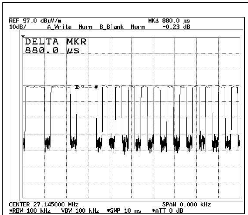
Duty Cycle 1
