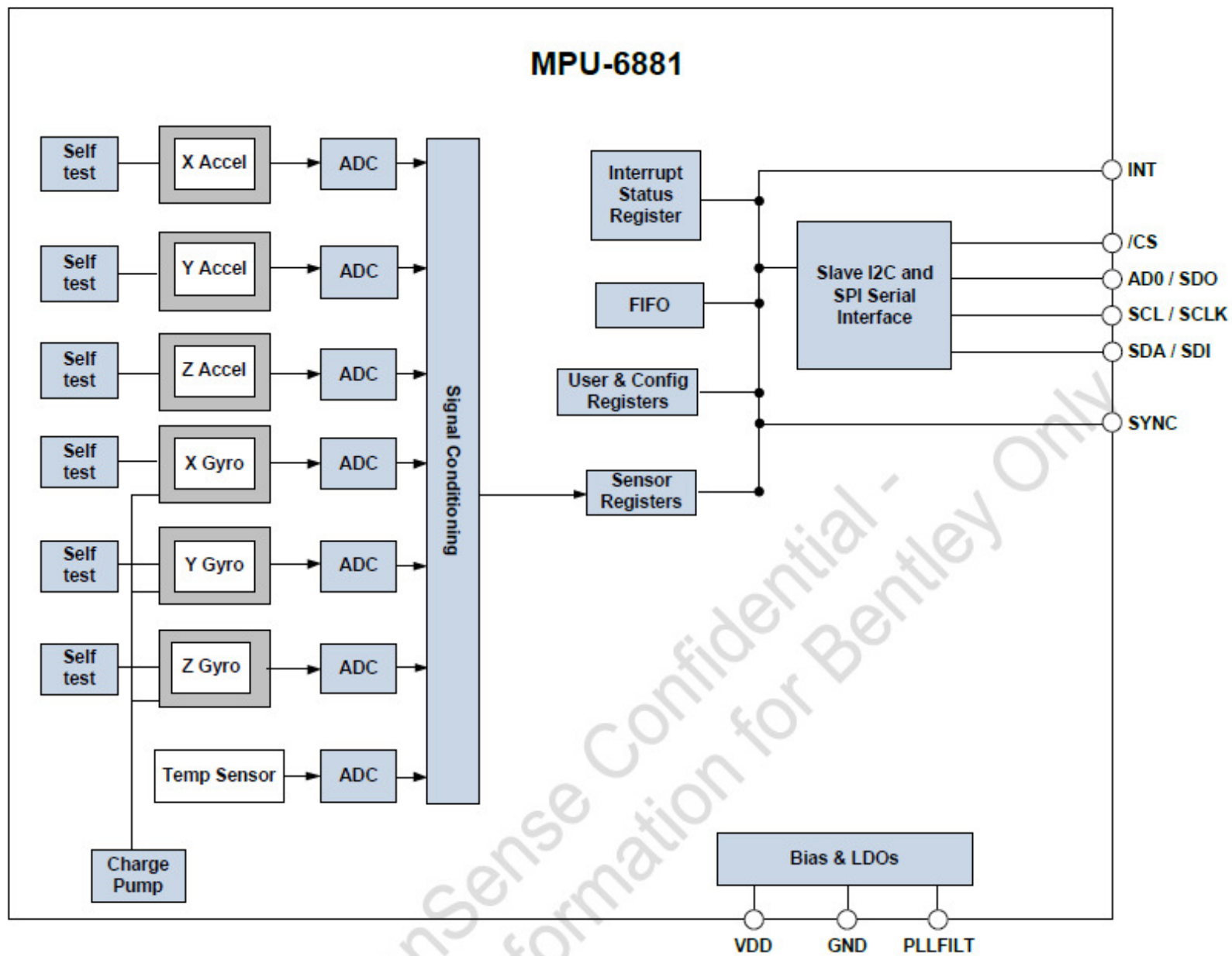
Figure 5 MPU-6881 Block Diagram
