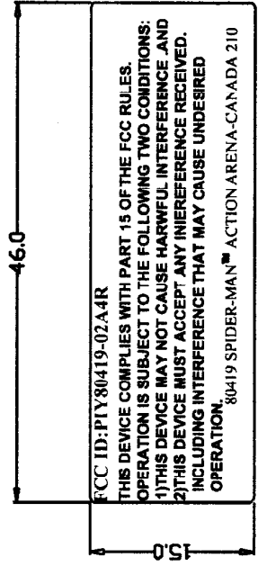
FCC LABEL SIZE 46MM X 15MM
