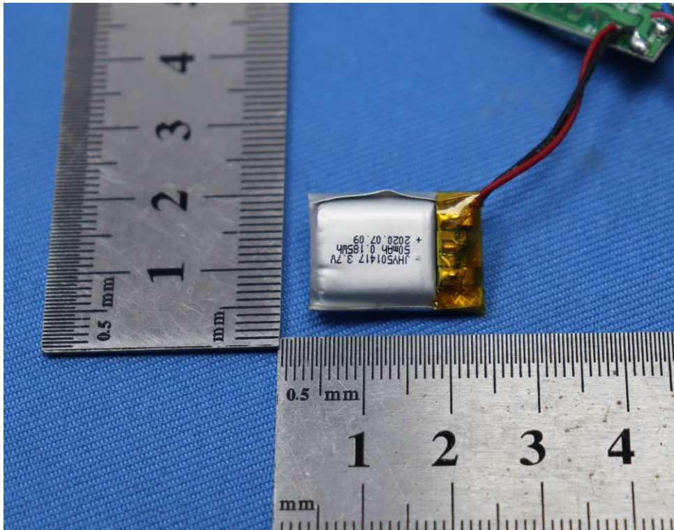
Rechargeable battery DC3.7V,50mAh
